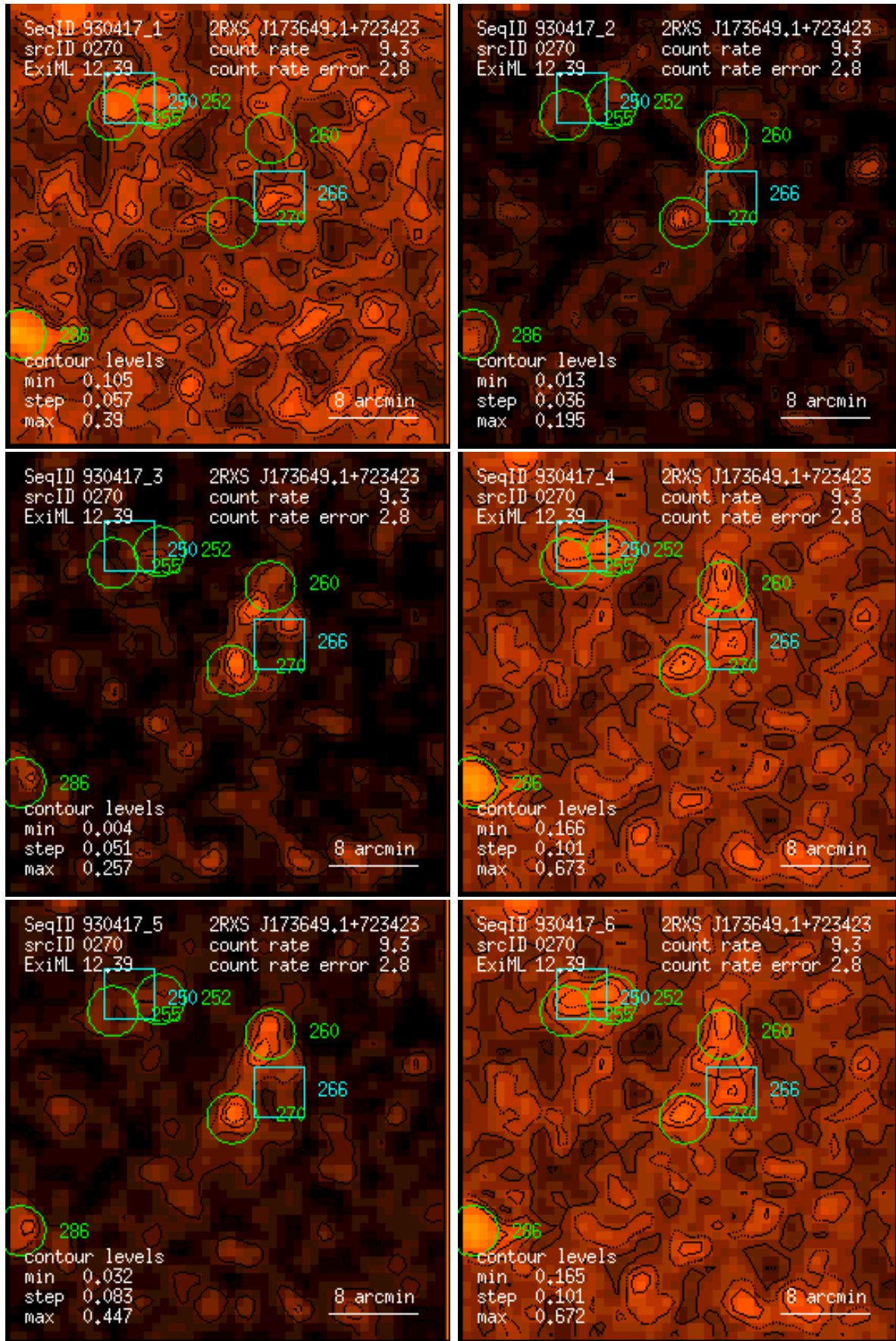
Figure 270: RASS 930417: detection 0270: band rate images, Gaussian filter: (1) PSPC channels 11 – 41, (2) 52 – 90, (3) 91 – 201, (4) 11 – 235, (5) 52 – 201, (6) 11 – 201. Broad band rates in counts/ks. Band rate contour levels in counts/ks/arcmin 2 .
