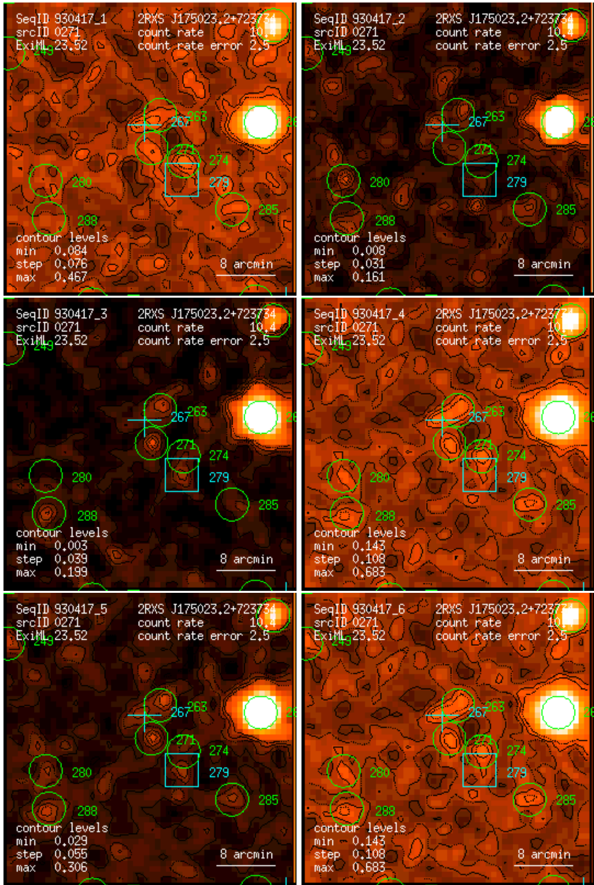
Figure 271: RASS 930417: detection 0271: band rate images, Gaussian filter: (1) PSPC channels 11 – 41, (2) 52 – 90, (3) 91 – 201, (4) 11 – 235, (5) 52 – 201, (6) 11 – 201. Broad band rates in counts/ks. Band rate contour levels in counts/ks/arcmin 2 .
