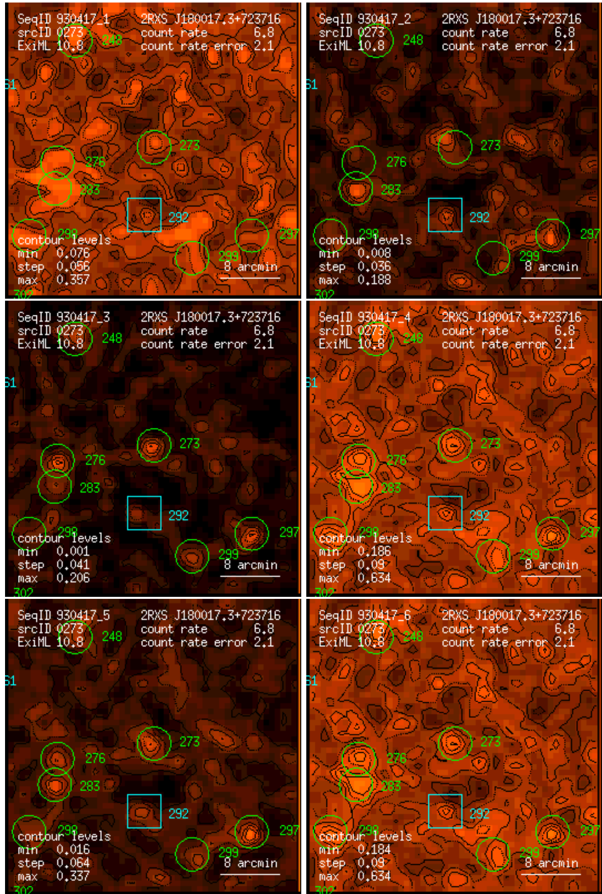
Figure 273: RASS 930417: detection 0273: band rate images, Gaussian filter: (1) PSPC channels 11 – 41, (2) 52 – 90, (3) 91 – 201, (4) 11 – 235, (5) 52 – 201, (6) 11 – 201. Broad band rates in counts/ks. Band rate contour levels in counts/ks/arcmin 2 .
