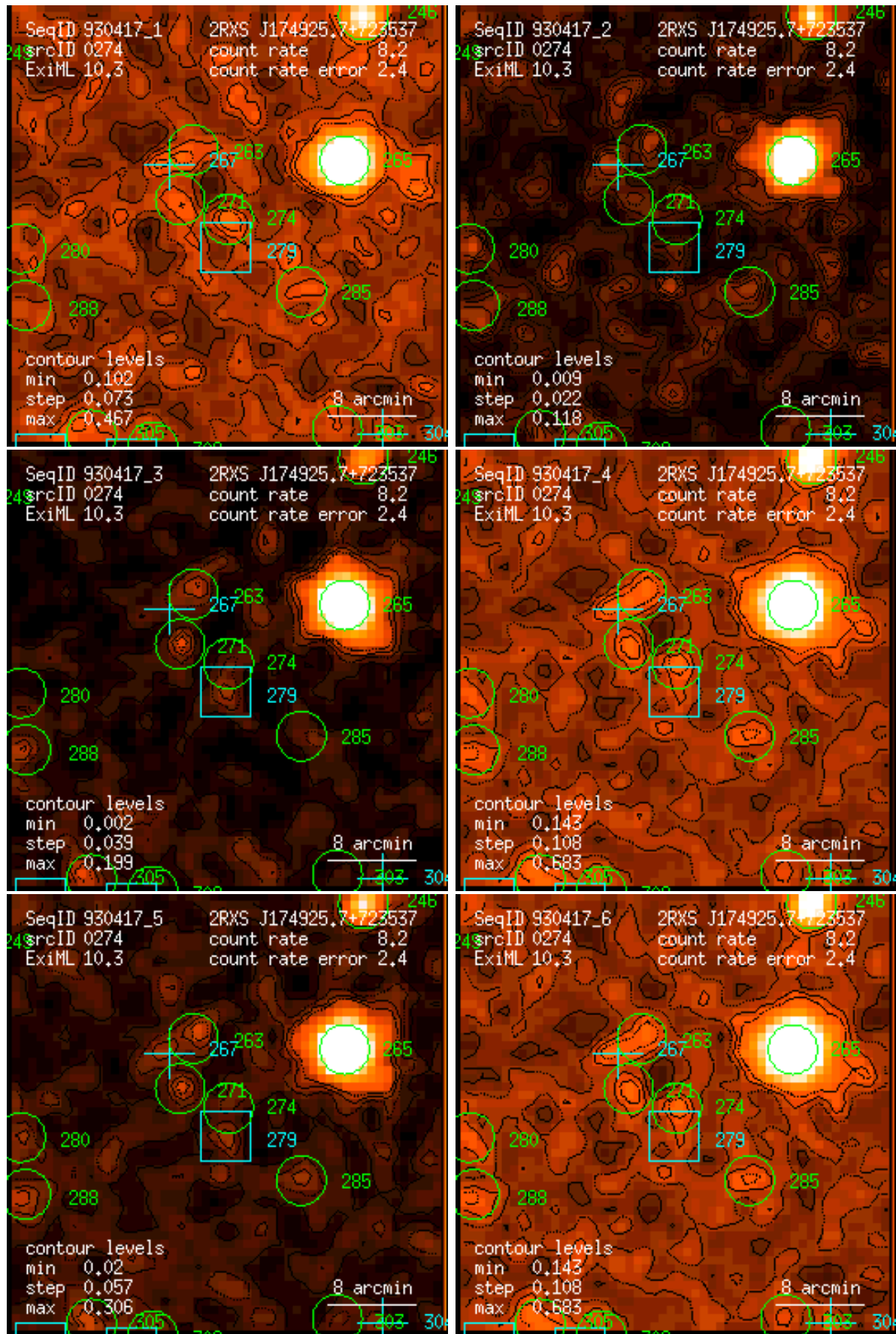
Figure 274: RASS 930417: detection 0274: band rate images, Gaussian filter: (1) PSPC channels 11 – 41, (2) 52 – 90, (3) 91 – 201, (4) 11 – 235, (5) 52 – 201, (6) 11 – 201. Broad band rates in counts/ks. Band rate contour levels in counts/ks/arcmin 2 .
