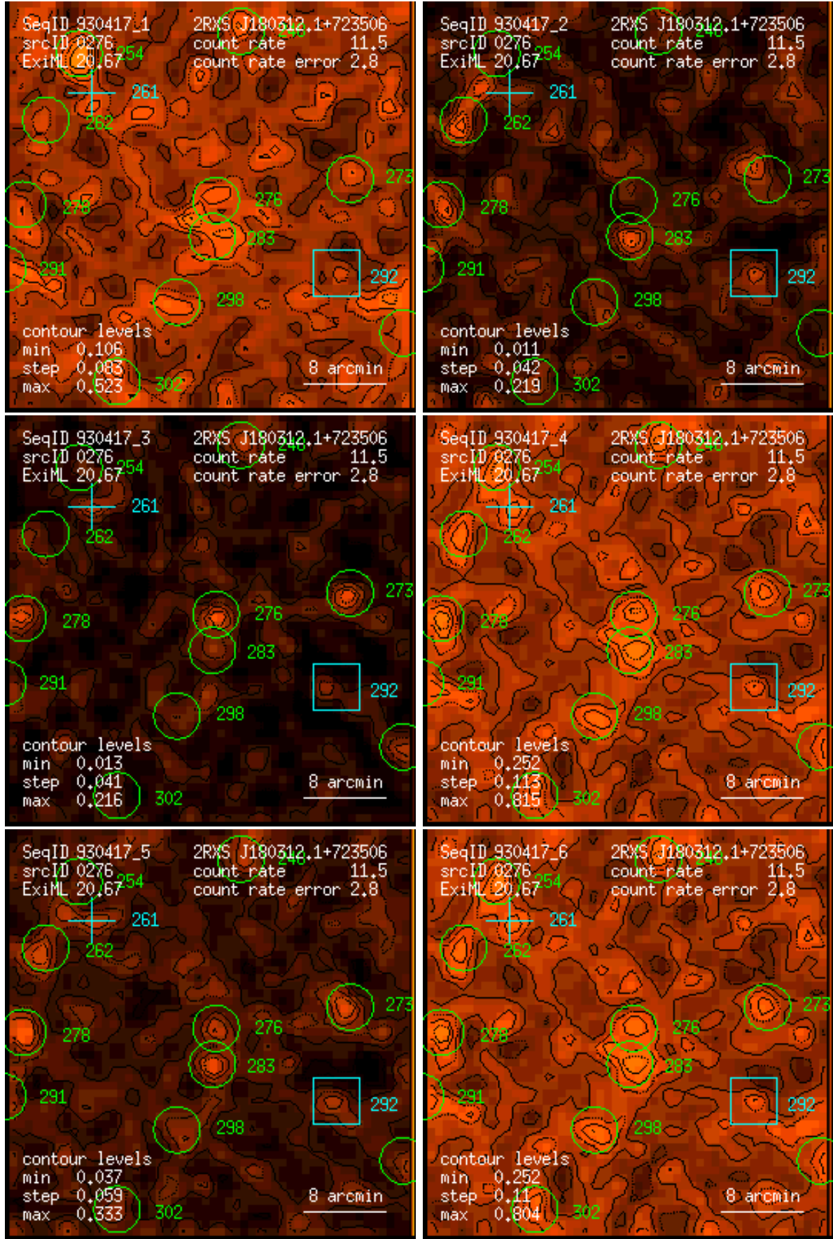
Figure 276: RASS 930417: detection 0276: band rate images, Gaussian filter: (1) PSPC channels 11 – 41, (2) 52 – 90, (3) 91 – 201, (4) 11 – 235, (5) 52 – 201, (6) 11 – 201. Broad band rates in counts/ks. Band rate contour levels in counts/ks/arcmin 2 .
