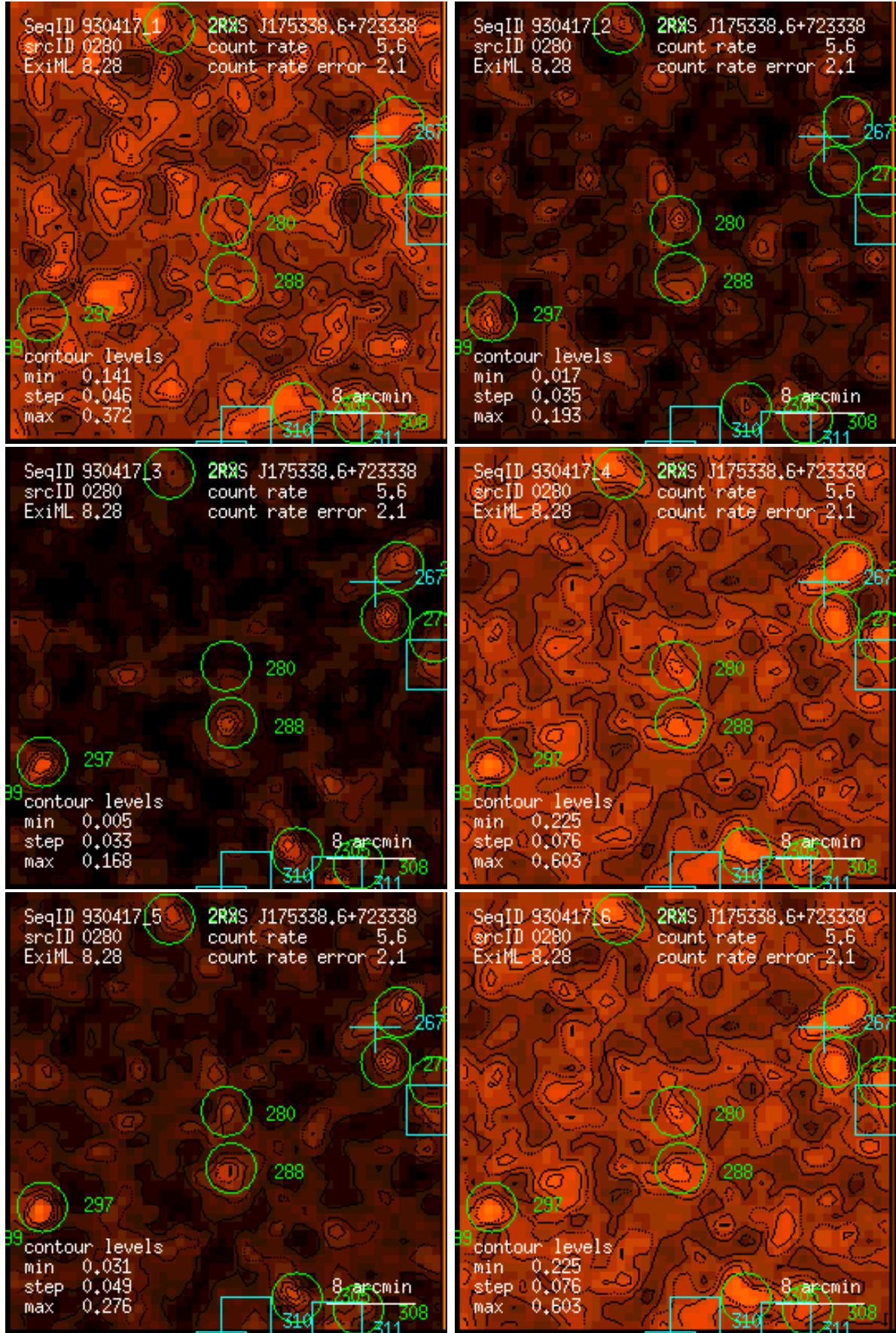
Figure 280: RASS 930417: detection 0280: band rate images, Gaussian filter: (1) PSPC channels 11 – 41, (2) 52 – 90, (3) 91 – 201, (4) 11 – 235, (5) 52 – 201, (6) 11 – 201. Broad band rates in counts/ks. Band rate contour levels in counts/ks/arcmin 2 .
