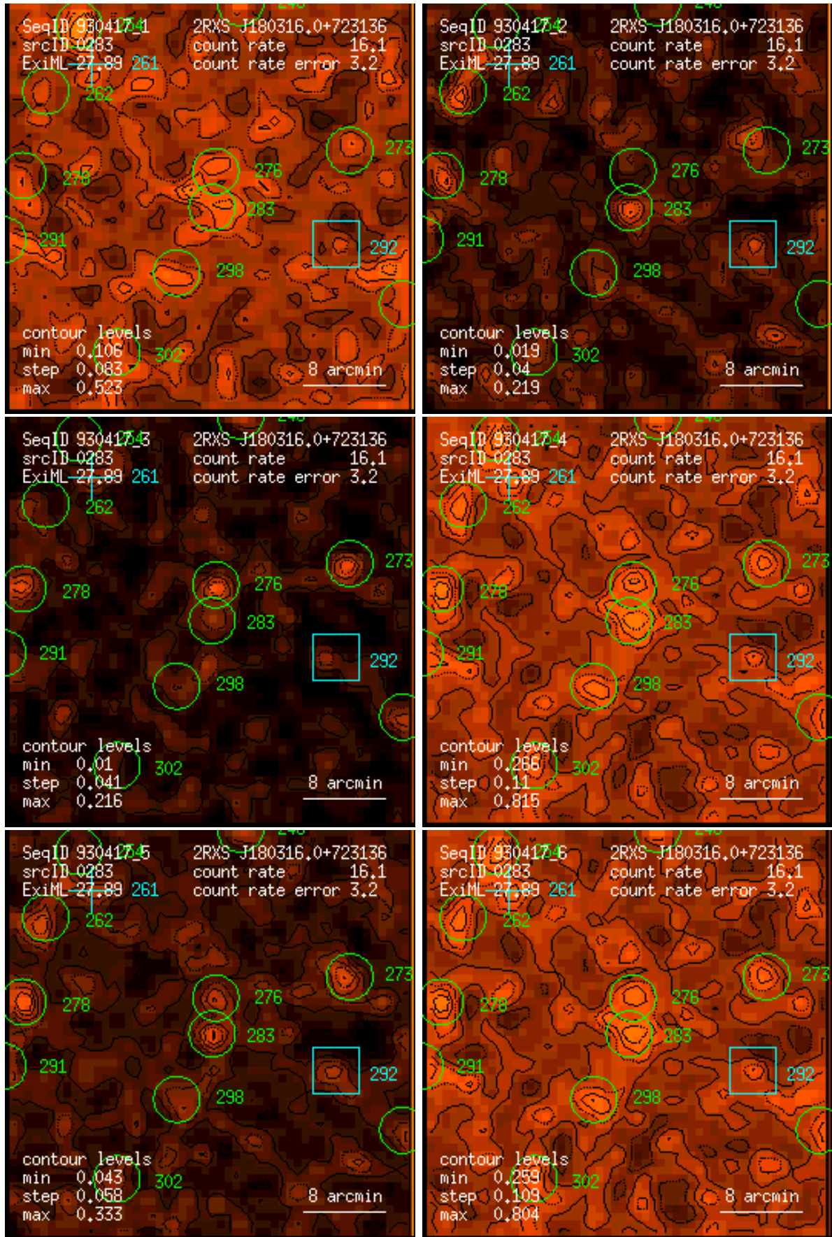
Figure 283: RASS 930417: detection 0283: band rate images, Gaussian filter: (1) PSPC channels 11 – 41, (2) 52 – 90, (3) 91 – 201, (4) 11 – 235, (5) 52 – 201, (6) 11 – 201. Broad band rates in counts/ks. Band rate contour levels in counts/ks/arcmin 2 .
