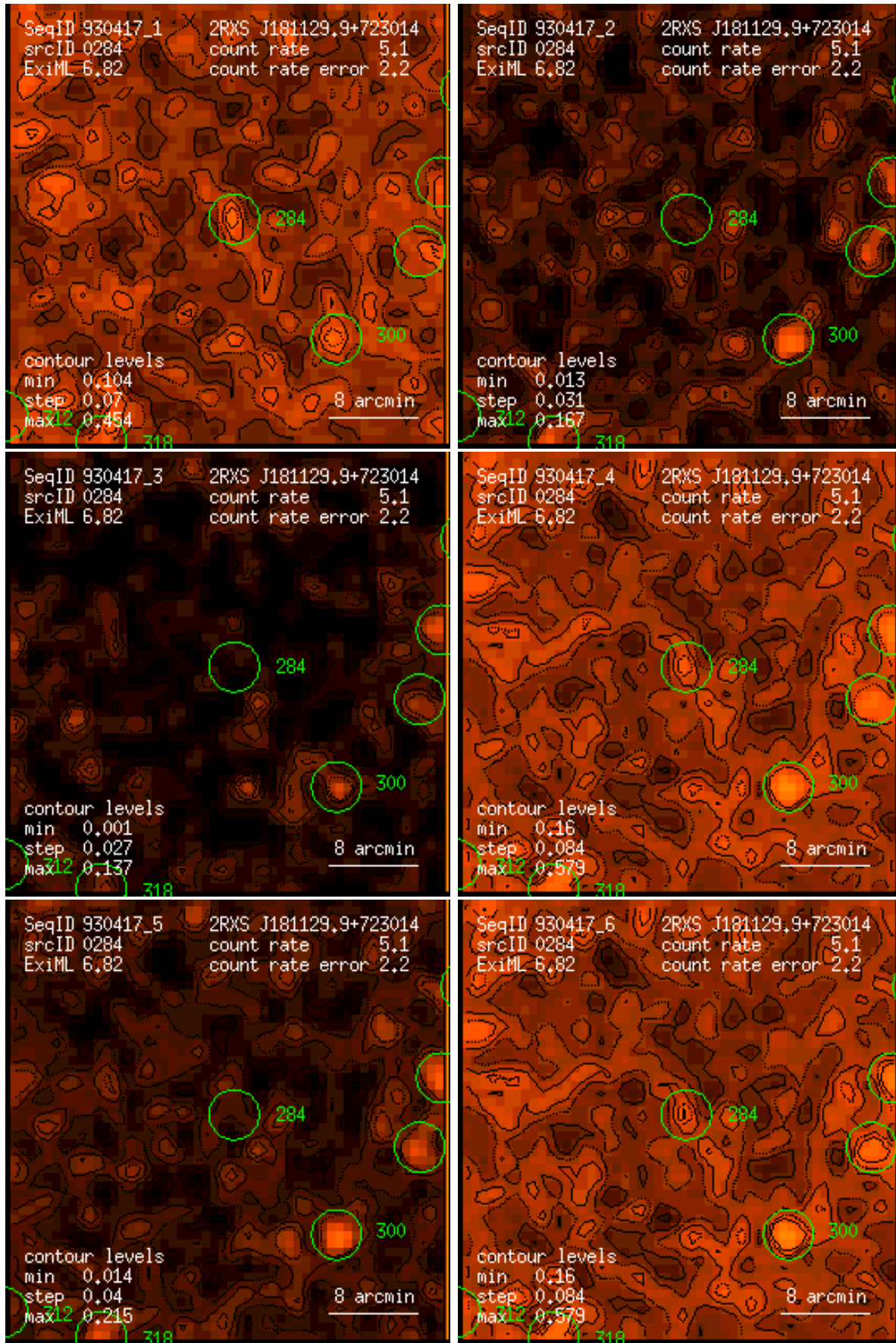
Figure 284: RASS 930417: detection 0284: band rate images, Gaussian filter: (1) PSPC channels 11 – 41, (2) 52 – 90, (3) 91 – 201, (4) 11 – 235, (5) 52 – 201, (6) 11 – 201. Broad band rates in counts/ks. Band rate contour levels in counts/ks/arcmin 2 .
