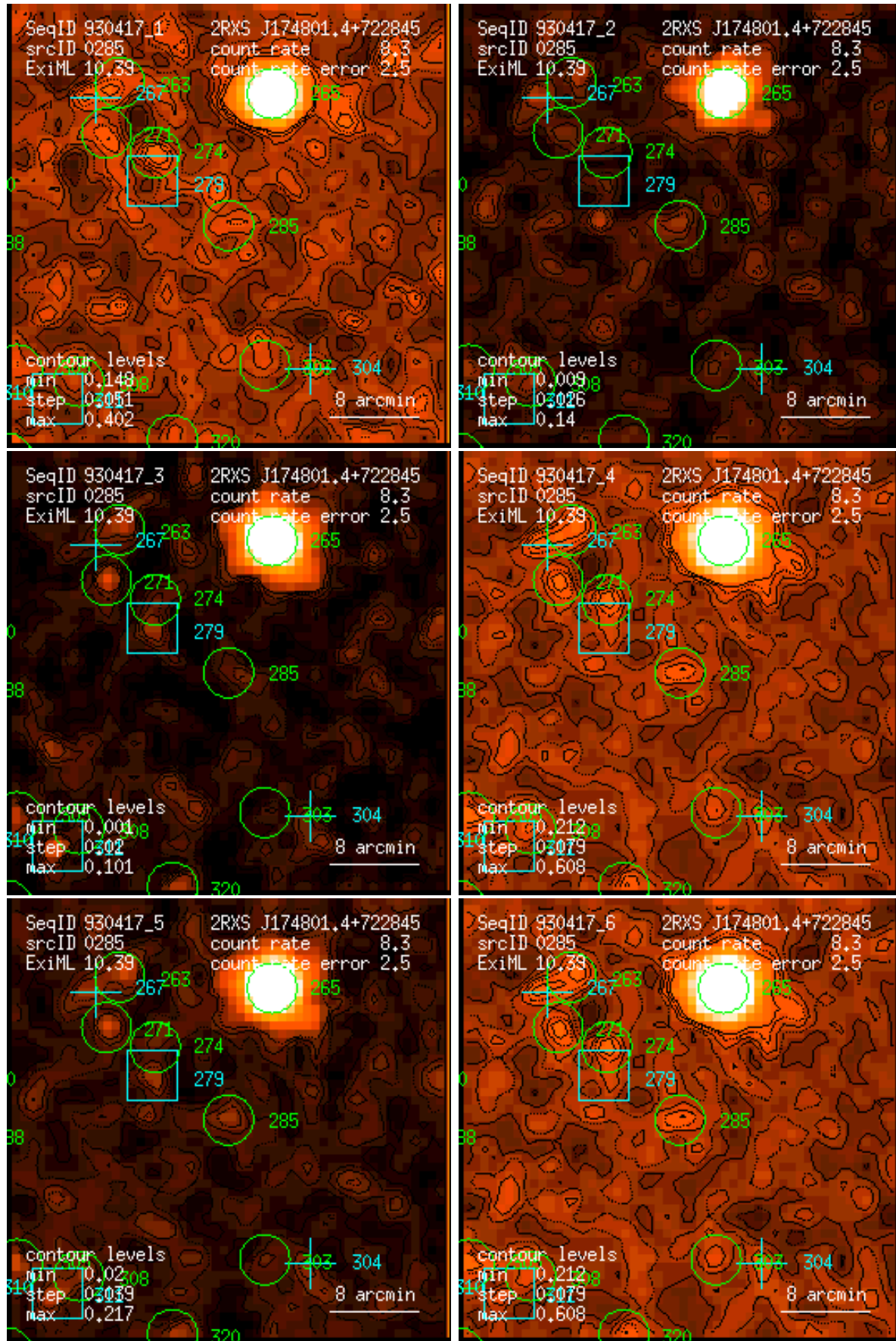
Figure 285: RASS 930417: detection 0285: band rate images, Gaussian filter: (1) PSPC channels 11 – 41, (2) 52 – 90, (3) 91 – 201, (4) 11 – 235, (5) 52 – 201, (6) 11 – 201. Broad band rates in counts/ks. Band rate contour levels in counts/ks/arcmin 2 .
