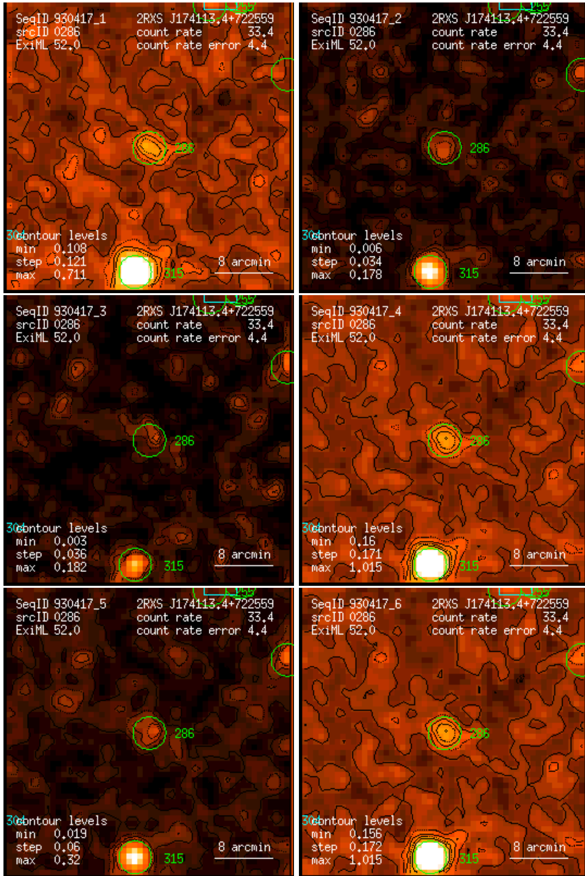
Figure 286: RASS 930417: detection 0286: band rate images, Gaussian filter: (1) PSPC channels 11 – 41, (2) 52 – 90, (3) 91 – 201, (4) 11 – 235, (5) 52 – 201, (6) 11 – 201. Broad band rates in counts/ks. Band rate contour levels in counts/ks/arcmin 2 .
