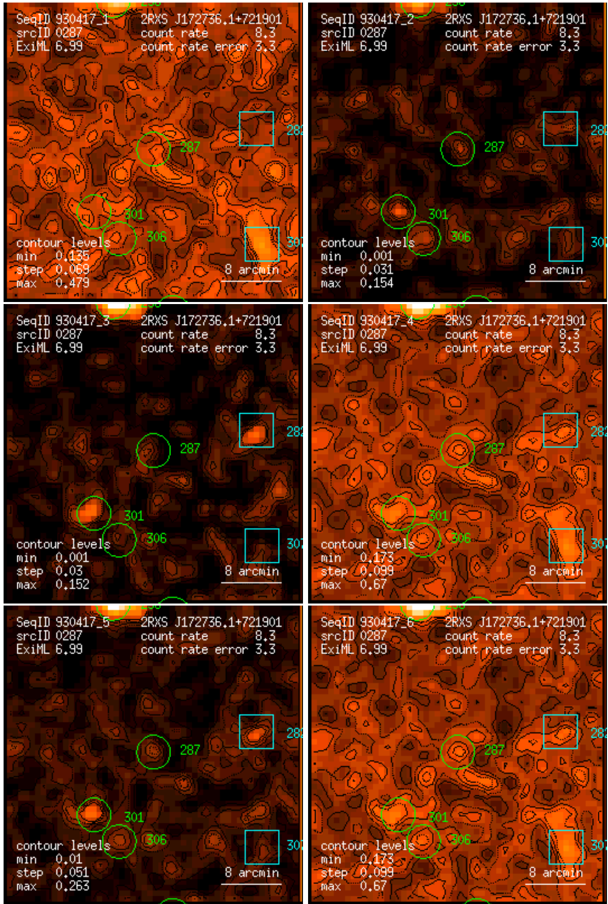
Figure 287: RASS 930417: detection 0287: band rate images, Gaussian filter: (1) PSPC channels 11 – 41, (2) 52 – 90, (3) 91 – 201, (4) 11 – 235, (5) 52 – 201, (6) 11 – 201. Broad band rates in counts/ks. Band rate contour levels in counts/ks/arcmin 2 .
