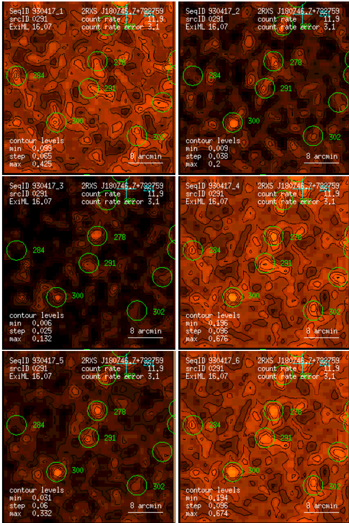
Figure 291: RASS 930417: detection 0291: band rate images, Gaussian filter: (1) PSPC channels 11 – 41, (2) 52 – 90, (3) 91 – 201, (4) 11 – 235, (5) 52 – 201, (6) 11 – 201. Broad band rates in counts/ks. Band rate contour levels in counts/ks/arcmin 2 .
