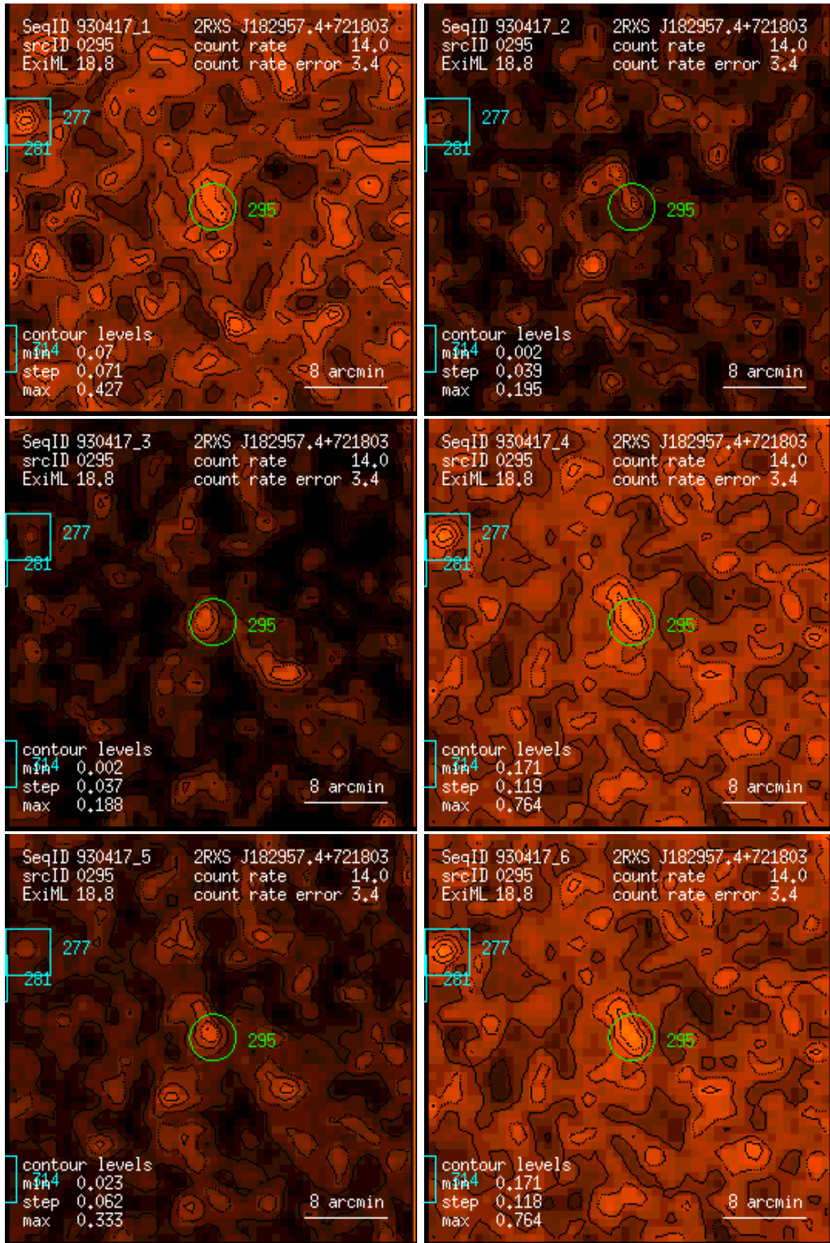
Figure 295: RASS 930417: detection 0295: band rate images, Gaussian filter: (1) PSPC channels 11 – 41, (2) 52 – 90, (3) 91 – 201, (4) 11 – 235, (5) 52 – 201, (6) 11 – 201. Broad band rates in counts/ks. Band rate contour levels in counts/ks/arcmin 2 .
