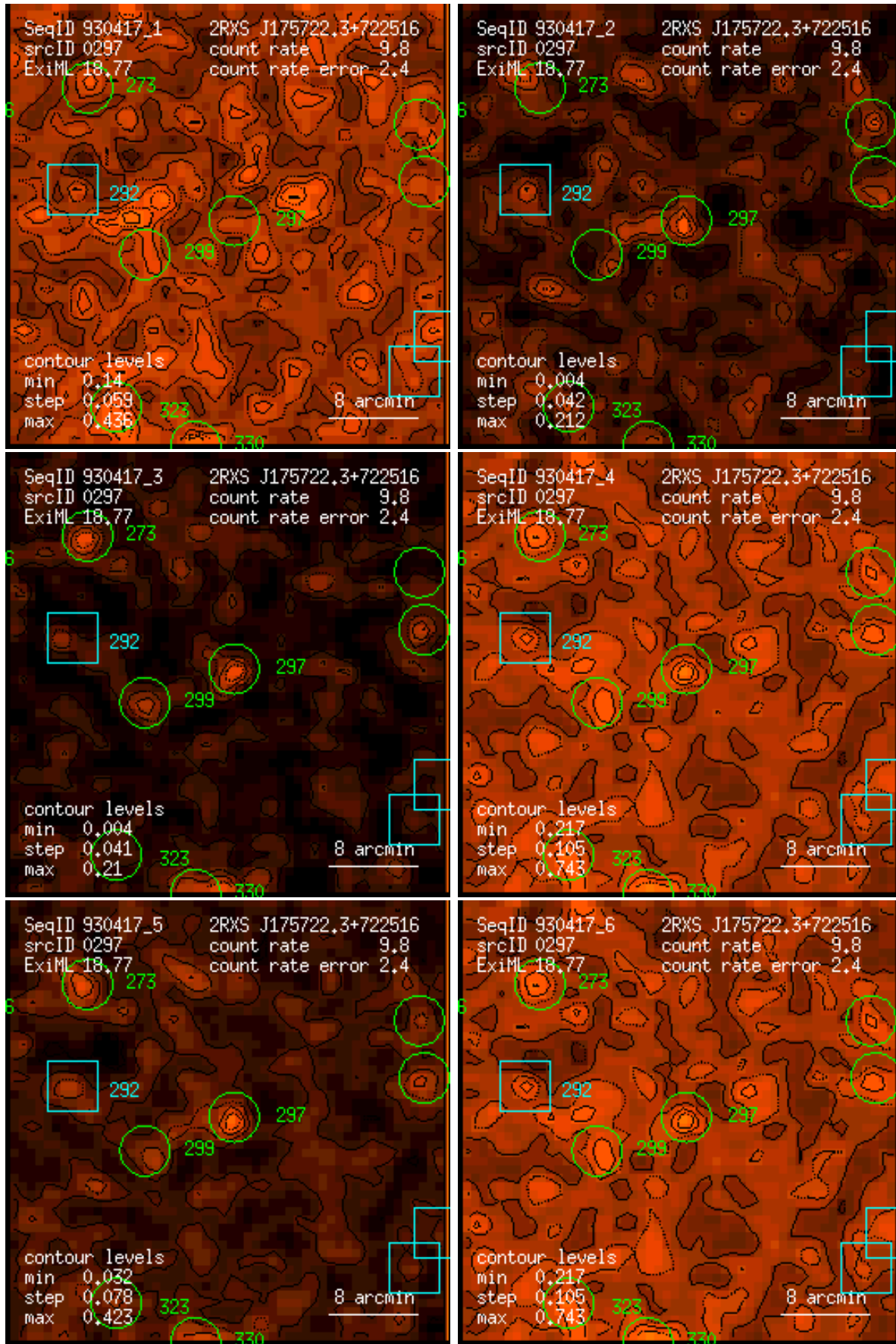
Figure 297: RASS 930417: detection 0297: band rate images, Gaussian filter: (1) PSPC channels 11 – 41, (2) 52 – 90, (3) 91 – 201, (4) 11 – 235, (5) 52 – 201, (6) 11 – 201. Broad band rates in counts/ks. Band rate contour levels in counts/ks/arcmin 2 .
