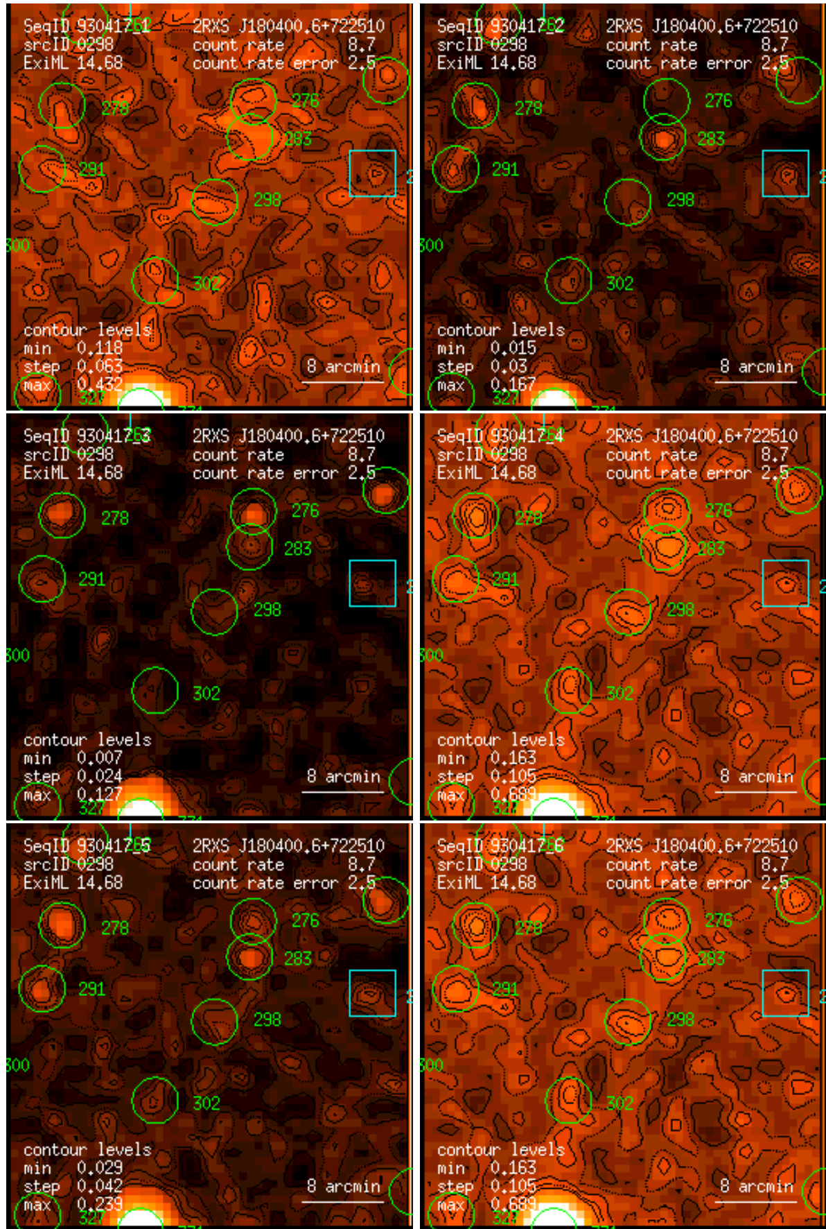
Figure 298: RASS 930417: detection 0298: band rate images, Gaussian filter: (1) PSPC channels 11 – 41, (2) 52 – 90, (3) 91 – 201, (4) 11 – 235, (5) 52 – 201, (6) 11 – 201. Broad band rates in counts/ks. Band rate contour levels in counts/ks/arcmin 2 .
