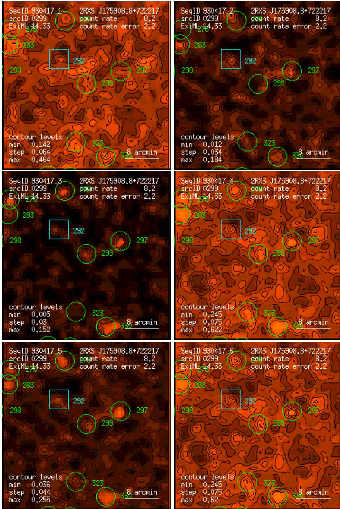
Figure 299: RASS 930417: detection 0299: band rate images, Gaussian filter: (1) PSPC channels 11 – 41, (2) 52 – 90, (3) 91 – 201, (4) 11 – 235, (5) 52 – 201, (6) 11 – 201. Broad band rates in counts/ks. Band rate contour levels in counts/ks/arcmin 2 .
