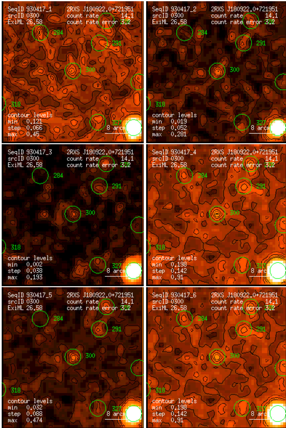
Figure 300: RASS 930417: detection 0300: band rate images, Gaussian filter: (1) PSPC channels 11 – 41, (2) 52 – 90, (3) 91 – 201, (4) 11 – 235, (5) 52 – 201, (6) 11 – 201. Broad band rates in counts/ks. Band rate contour levels in counts/ks/arcmin 2 .
