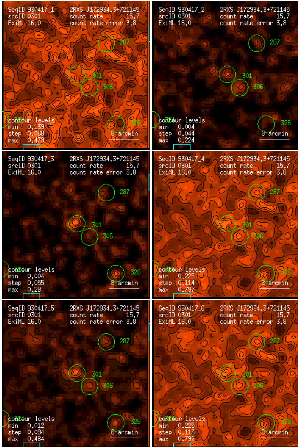
Figure 301: RASS 930417: detection 0301: band rate images, Gaussian filter: (1) PSPC channels 11 – 41, (2) 52 – 90, (3) 91 – 201, (4) 11 – 235, (5) 52 – 201, (6) 11 – 201. Broad band rates in counts/ks. Band rate contour levels in counts/ks/arcmin 2 .
