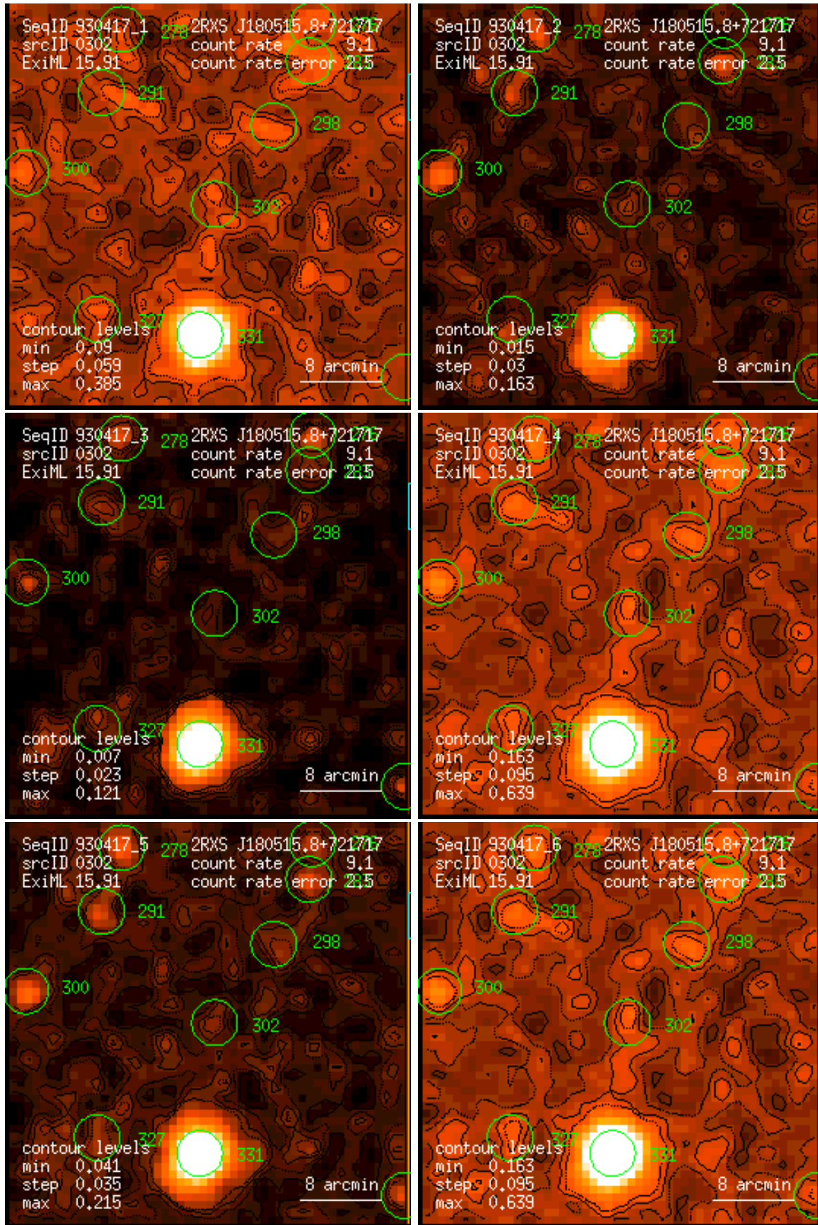
Figure 302: RASS 930417: detection 0302: band rate images, Gaussian filter: (1) PSPC channels 11 – 41, (2) 52 – 90, (3) 91 – 201, (4) 11 – 235, (5) 52 – 201, (6) 11 – 201. Broad band rates in counts/ks. Band rate contour levels in counts/ks/arcmin 2 .
