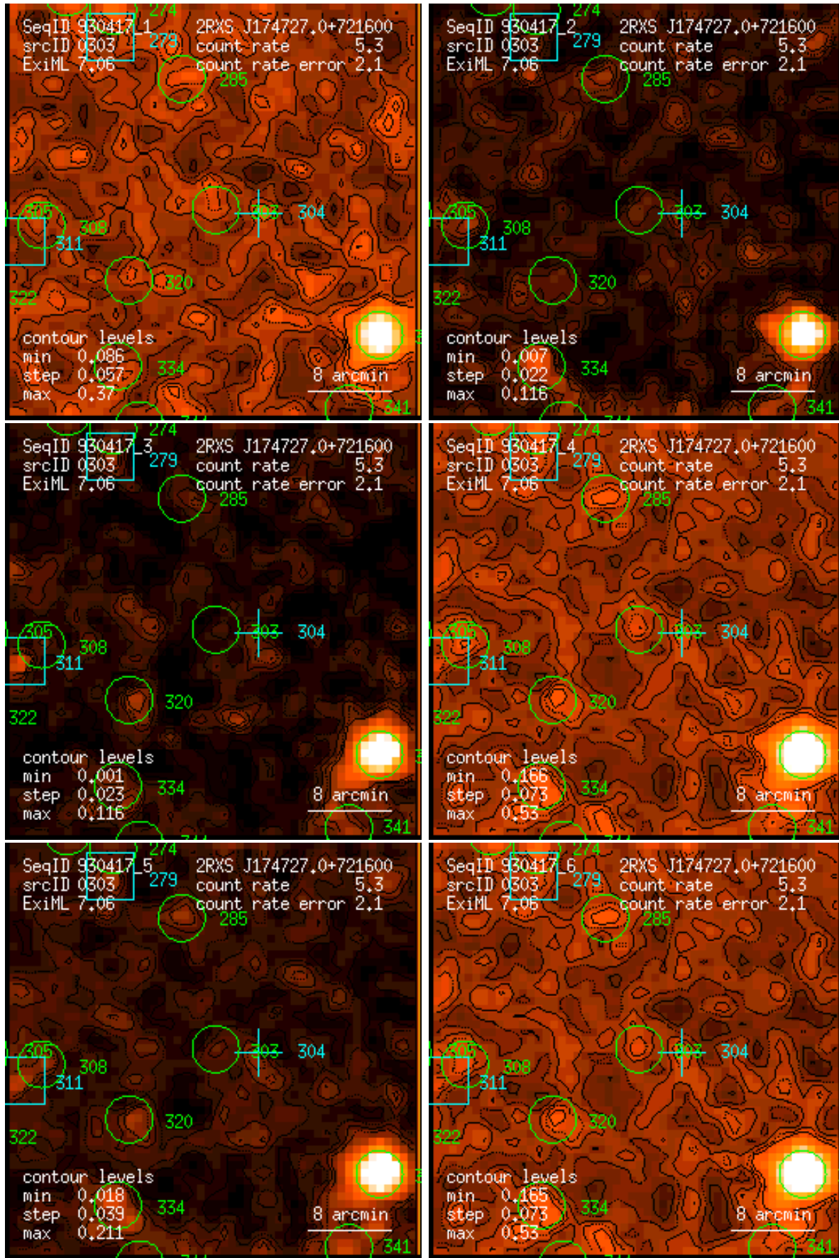
Figure 303: RASS 930417: detection 0303: band rate images, Gaussian filter: (1) PSPC channels 11 – 41, (2) 52 – 90, (3) 91 – 201, (4) 11 – 235, (5) 52 – 201, (6) 11 – 201. Broad band rates in counts/ks. Band rate contour levels in counts/ks/arcmin 2 .
