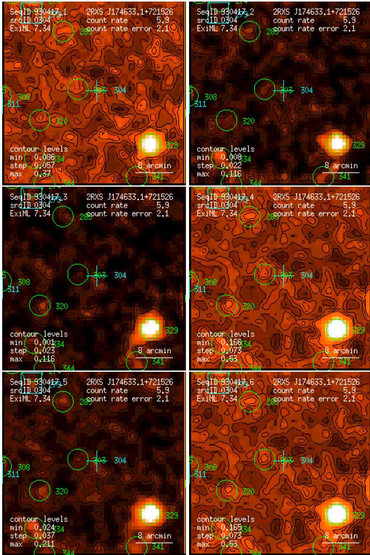
Figure 304: RASS 930417: detection 0304: band rate images, Gaussian filter: (1) PSPC channels 11 – 41, (2) 52 – 90, (3) 91 – 201, (4) 11 – 235, (5) 52 – 201, (6) 11 – 201. Broad band rates in counts/ks. Band rate contour levels in counts/ks/arcmin 2 .
