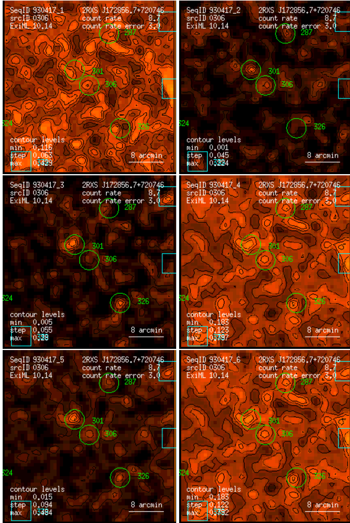
Figure 306: RASS 930417: detection 0306: band rate images, Gaussian filter: (1) PSPC channels 11 – 41, (2) 52 – 90, (3) 91 – 201, (4) 11 – 235, (5) 52 – 201, (6) 11 – 201. Broad band rates in counts/ks. Band rate contour levels in counts/ks/arcmin 2 .
