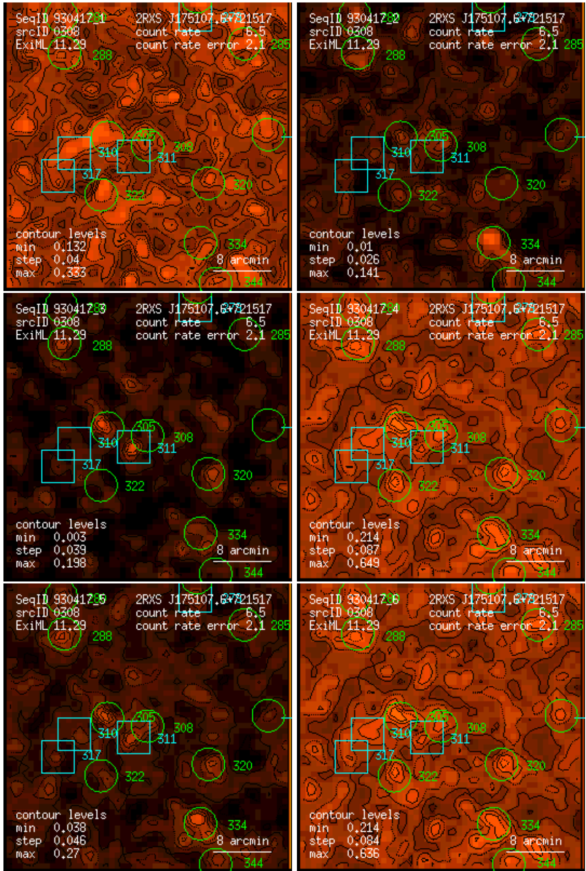
Figure 308: RASS 930417: detection 0308: band rate images, Gaussian filter: (1) PSPC channels 11 – 41, (2) 52 – 90, (3) 91 – 201, (4) 11 – 235, (5) 52 – 201, (6) 11 – 201. Broad band rates in counts/ks. Band rate contour levels in counts/ks/arcmin 2 .
