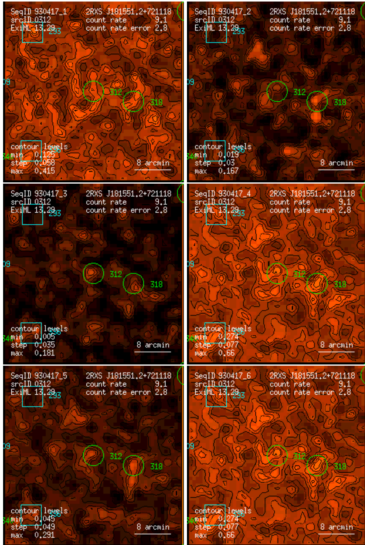
Figure 312: RASS 930417: detection 0312: band rate images, Gaussian filter: (1) PSPC channels 11 – 41, (2) 52 – 90, (3) 91 – 201, (4) 11 – 235, (5) 52 – 201, (6) 11 – 201. Broad band rates in counts/ks. Band rate contour levels in counts/ks/arcmin 2 .
