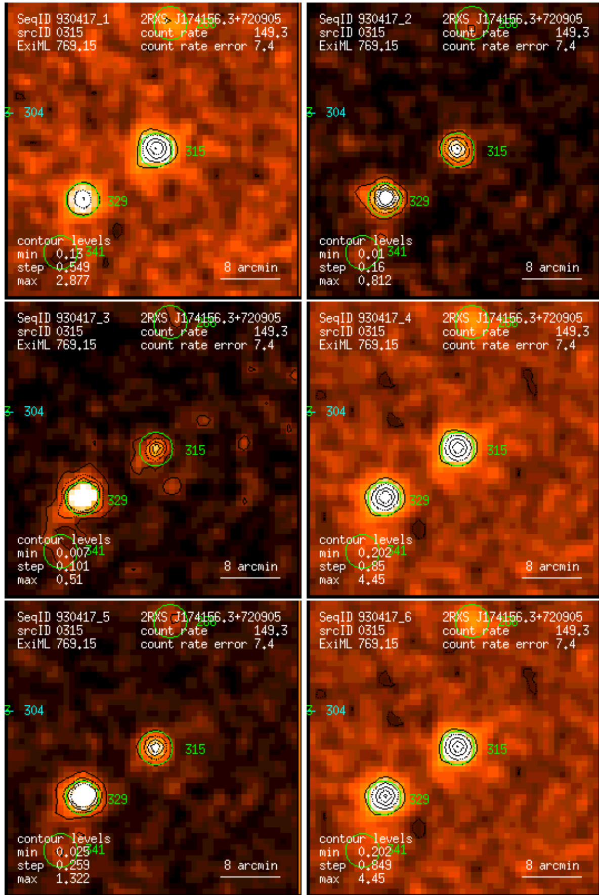
Figure 315: RASS 930417: detection 0315: band rate images, Gaussian filter: (1) PSPC channels 11 – 41, (2) 52 – 90, (3) 91 – 201, (4) 11 – 235, (5) 52 – 201, (6) 11 – 201. Broad band rates in counts/ks. Band rate contour levels in counts/ks/arcmin 2 .
