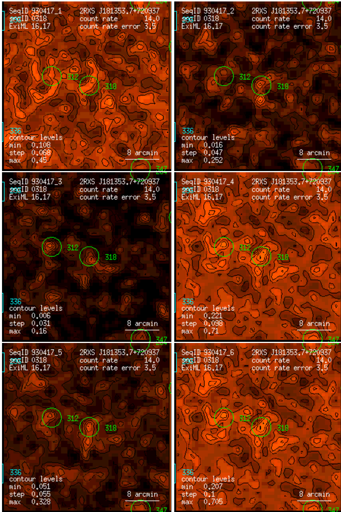
Figure 318: RASS 930417: detection 0318: band rate images, Gaussian filter: (1) PSPC channels 11 – 41, (2) 52 – 90, (3) 91 – 201, (4) 11 – 235, (5) 52 – 201, (6) 11 – 201. Broad band rates in counts/ks. Band rate contour levels in counts/ks/arcmin 2 .
