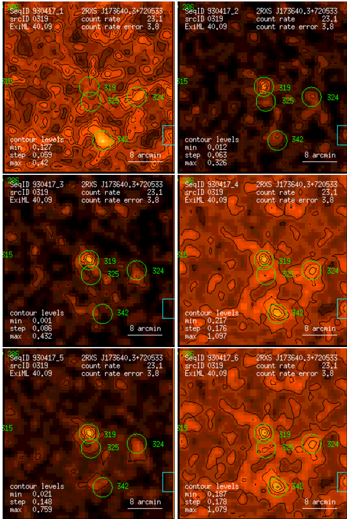
Figure 319: RASS 930417: detection 0319: band rate images, Gaussian filter: (1) PSPC channels 11 – 41, (2) 52 – 90, (3) 91 – 201, (4) 11 – 235, (5) 52 – 201, (6) 11 – 201. Broad band rates in counts/ks. Band rate contour levels in counts/ks/arcmin 2 .
