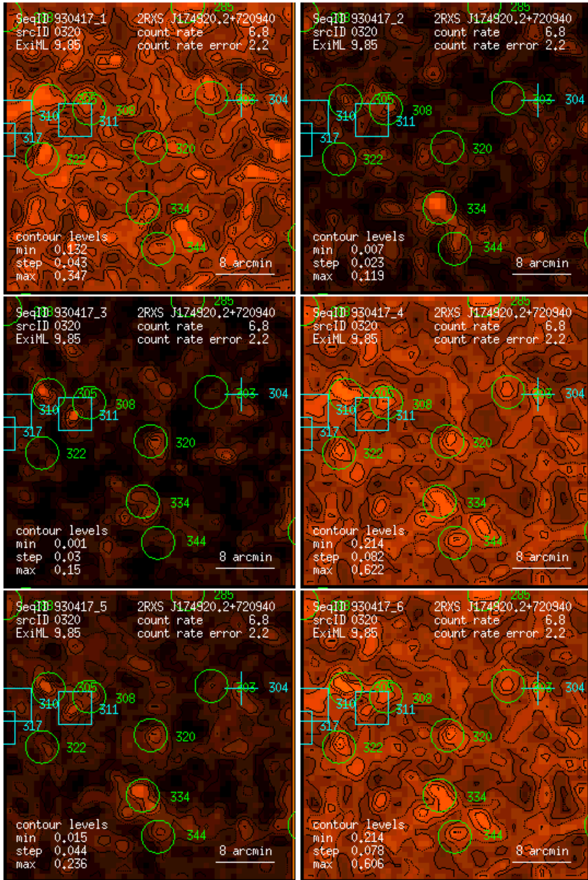
Figure 320: RASS 930417: detection 0320: band rate images, Gaussian filter: (1) PSPC channels 11 – 41, (2) 52 – 90, (3) 91 – 201, (4) 11 – 235, (5) 52 – 201, (6) 11 – 201. Broad band rates in counts/ks. Band rate contour levels in counts/ks/arcmin 2 .
