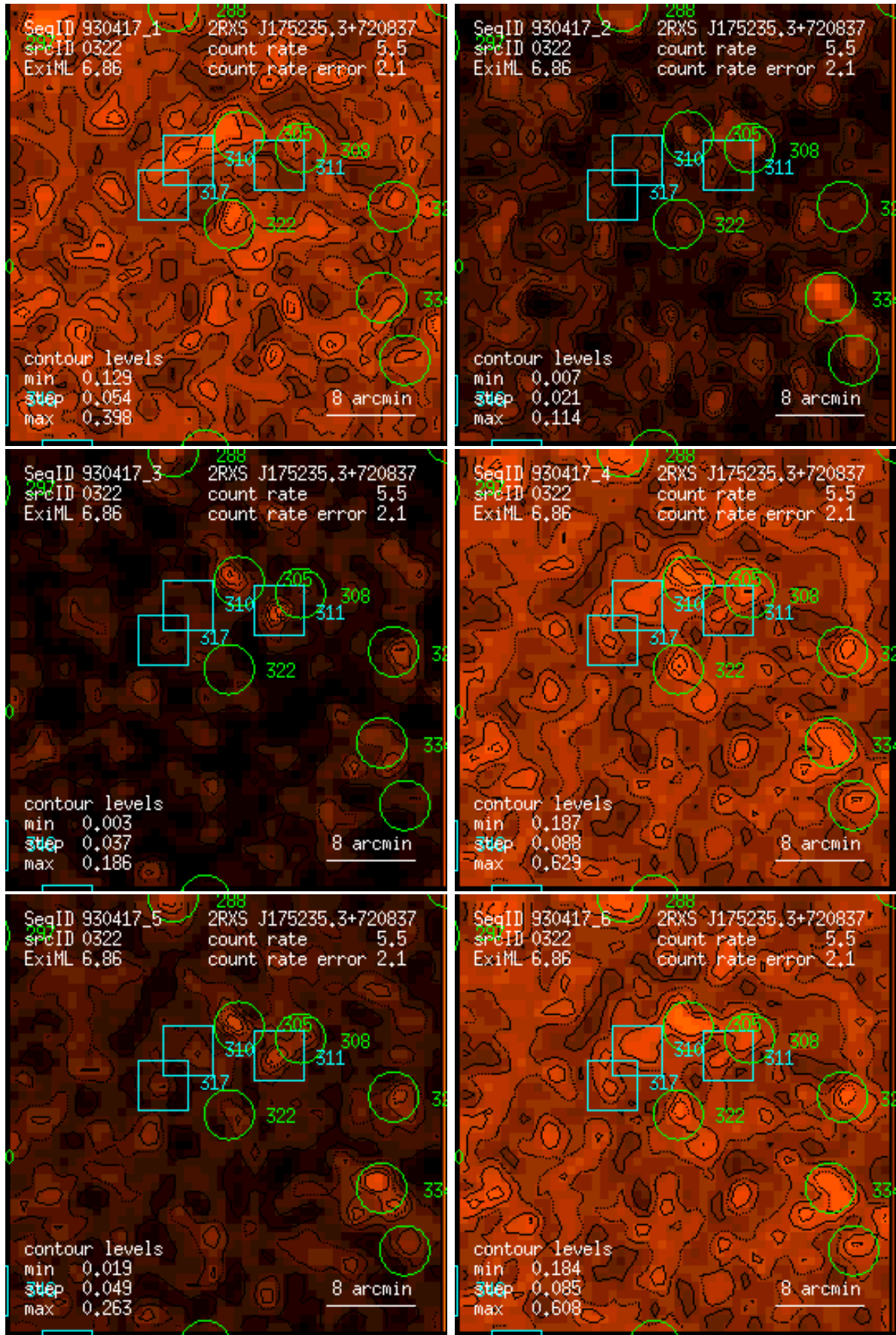
Figure 322: RASS 930417: detection 0322: band rate images, Gaussian filter: (1) PSPC channels 11 – 41, (2) 52 – 90, (3) 91 – 201, (4) 11 – 235, (5) 52 – 201, (6) 11 – 201. Broad band rates in counts/ks. Band rate contour levels in counts/ks/arcmin 2 .
