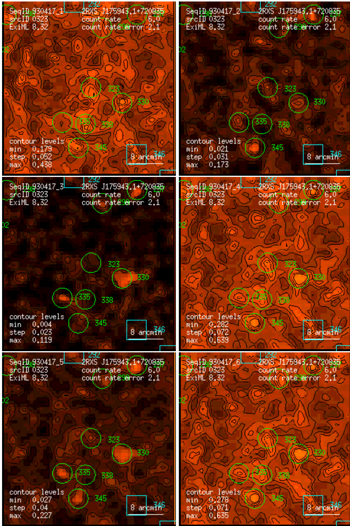
Figure 323: RASS 930417: detection 0323: band rate images, Gaussian filter: (1) PSPC channels 11 – 41, (2) 52 – 90, (3) 91 – 201, (4) 11 – 235, (5) 52 – 201, (6) 11 – 201. Broad band rates in counts/ks. Band rate contour levels in counts/ks/arcmin 2 .
