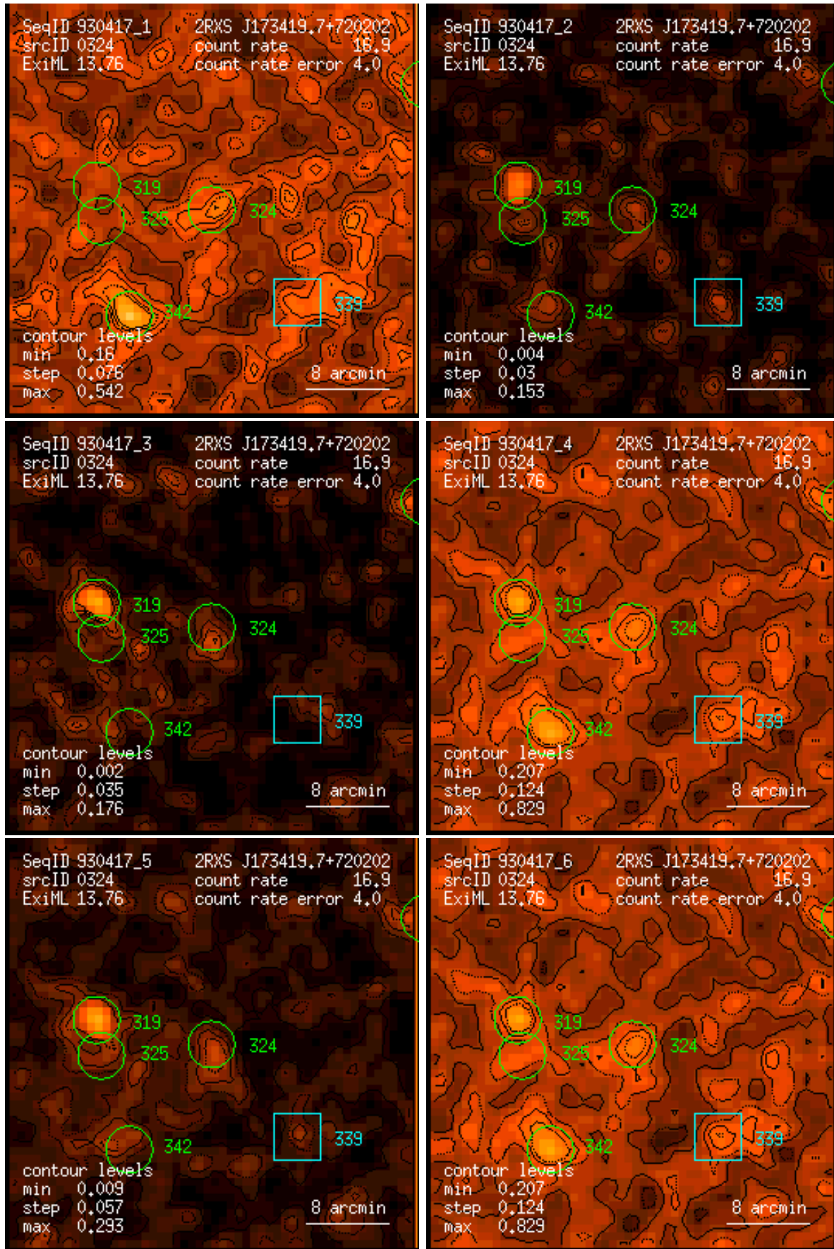
Figure 324: RASS 930417: detection 0324: band rate images, Gaussian filter: (1) PSPC channels 11 – 41, (2) 52 – 90, (3) 91 – 201, (4) 11 – 235, (5) 52 – 201, (6) 11 – 201. Broad band rates in counts/ks. Band rate contour levels in counts/ks/arcmin 2 .
