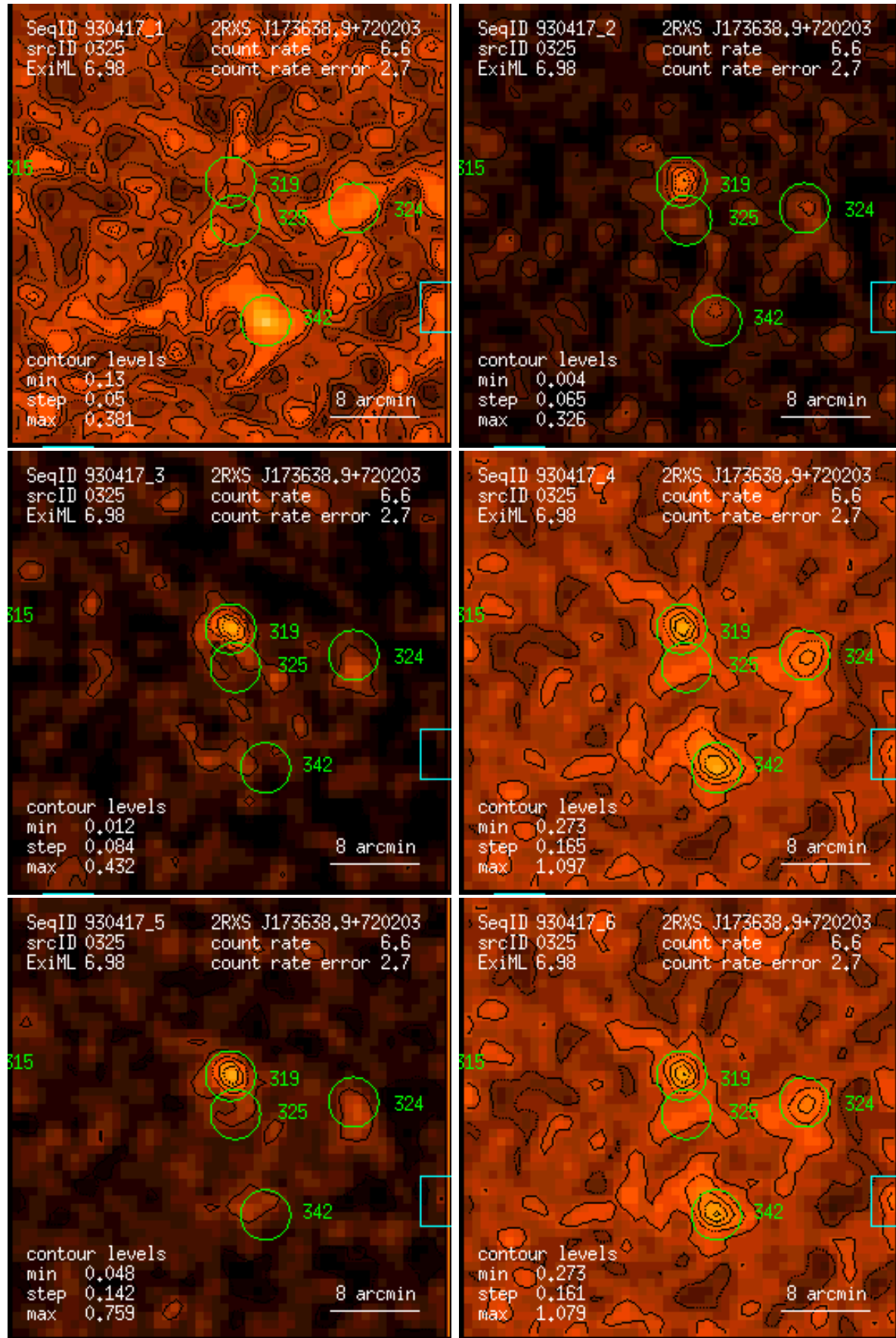
Figure 325: RASS 930417: detection 0325: band rate images, Gaussian filter: (1) PSPC channels 11 – 41, (2) 52 – 90, (3) 91 – 201, (4) 11 – 235, (5) 52 – 201, (6) 11 – 201. Broad band rates in counts/ks. Band rate contour levels in counts/ks/arcmin 2 .
