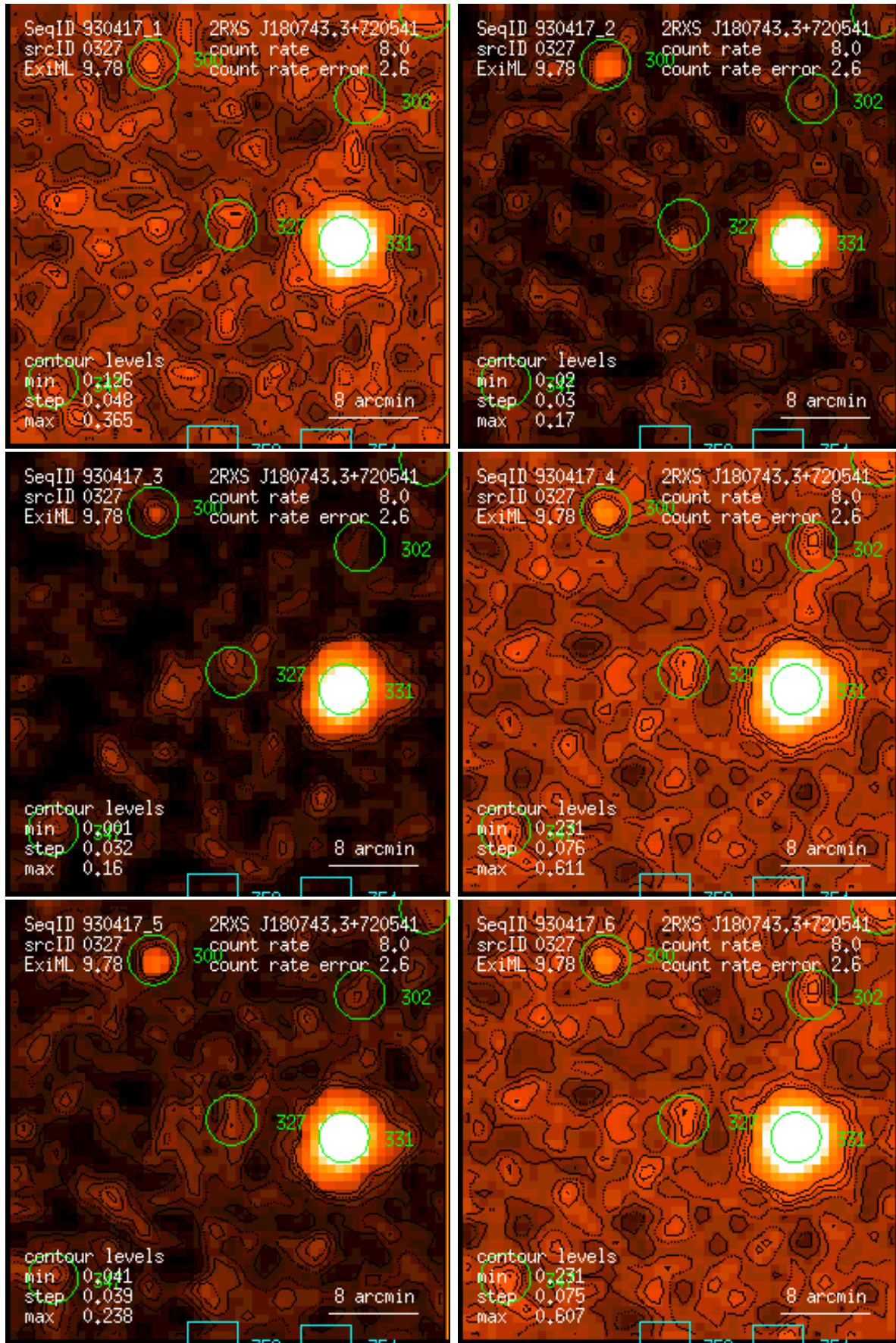
Figure 327: RASS 930417: detection 0327: band rate images, Gaussian filter: (1) PSPC channels 11 – 41, (2) 52 – 90, (3) 91 – 201, (4) 11 – 235, (5) 52 – 201, (6) 11 – 201. Broad band rates in counts/ks. Band rate contour levels in counts/ks/arcmin 2 .
