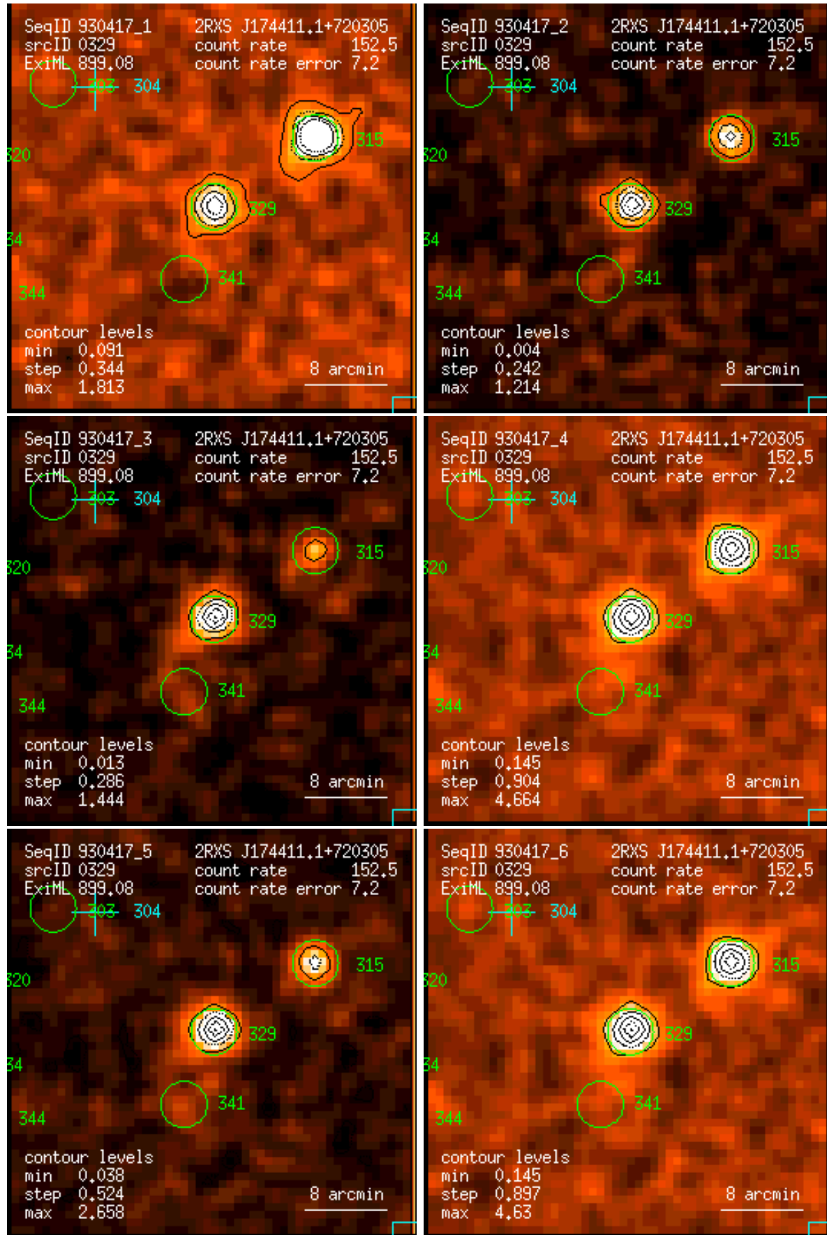
Figure 329: RASS 930417: detection 0329: band rate images, Gaussian filter: (1) PSPC channels 11 – 41, (2) 52 – 90, (3) 91 – 201, (4) 11 – 235, (5) 52 – 201, (6) 11 – 201. Broad band rates in counts/ks. Band rate contour levels in counts/ks/arcmin 2 .
