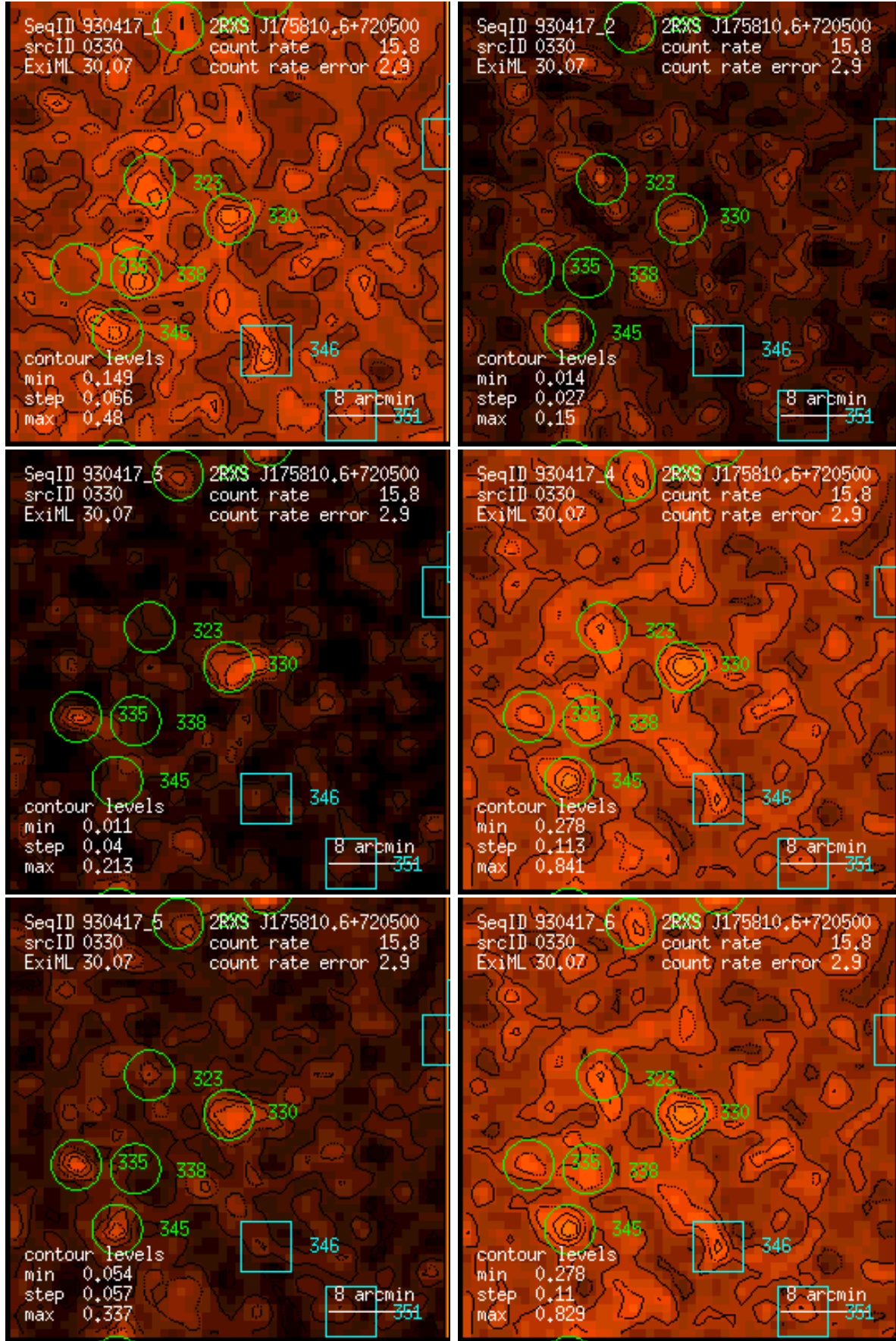
Figure 330: RASS 930417: detection 0330: band rate images, Gaussian filter: (1) PSPC channels 11 – 41, (2) 52 – 90, (3) 91 – 201, (4) 11 – 235, (5) 52 – 201, (6) 11 – 201. Broad band rates in counts/ks. Band rate contour levels in counts/ks/arcmin 2 .
