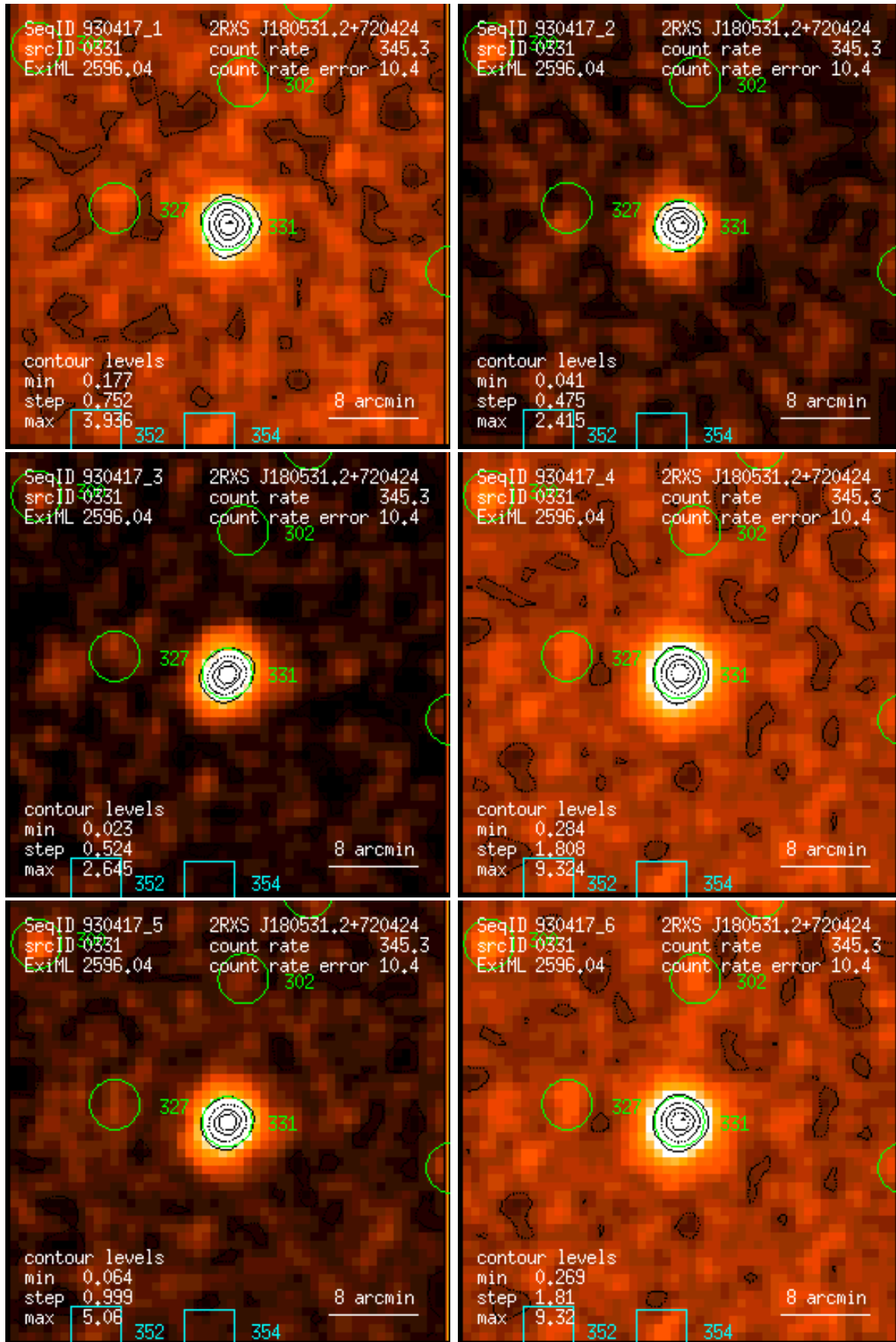
Figure 331: RASS 930417: detection 0331: band rate images, Gaussian filter: (1) PSPC channels 11 – 41, (2) 52 – 90, (3) 91 – 201, (4) 11 – 235, (5) 52 – 201, (6) 11 – 201. Broad band rates in counts/ks. Band rate contour levels in counts/ks/arcmin 2 .
