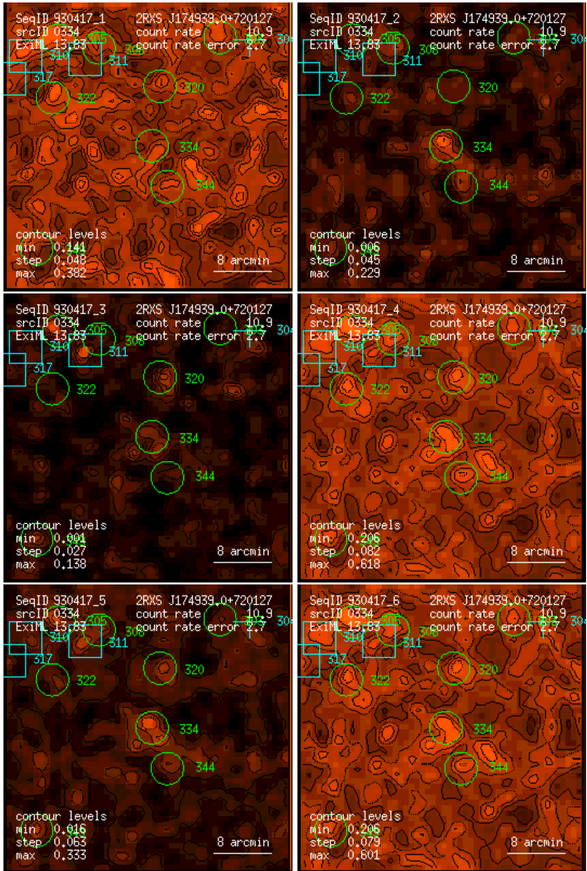
Figure 334: RASS 930417: detection 0334: band rate images, Gaussian filter: (1) PSPC channels 11 – 41, (2) 52 – 90, (3) 91 – 201, (4) 11 – 235, (5) 52 – 201, (6) 11 – 201. Broad band rates in counts/ks. Band rate contour levels in counts/ks/arcmin 2 .
