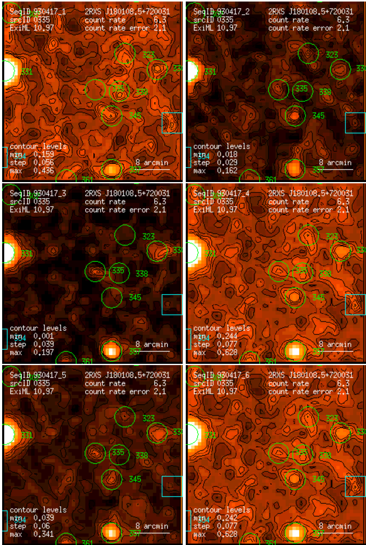
Figure 335: RASS 930417: detection 0335: band rate images, Gaussian filter: (1) PSPC channels 11 – 41, (2) 52 – 90, (3) 91 – 201, (4) 11 – 235, (5) 52 – 201, (6) 11 – 201. Broad band rates in counts/ks. Band rate contour levels in counts/ks/arcmin 2 .
