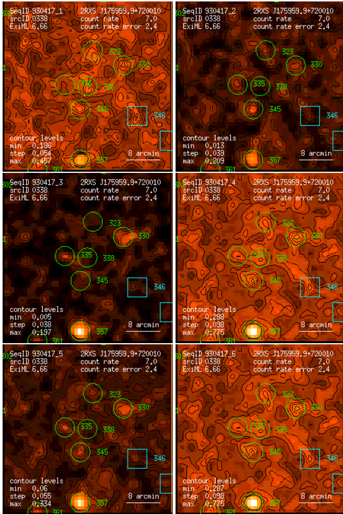
Figure 338: RASS 930417: detection 0338: band rate images, Gaussian filter: (1) PSPC channels 11 – 41, (2) 52 – 90, (3) 91 – 201, (4) 11 – 235, (5) 52 – 201, (6) 11 – 201. Broad band rates in counts/ks. Band rate contour levels in counts/ks/arcmin 2 .
