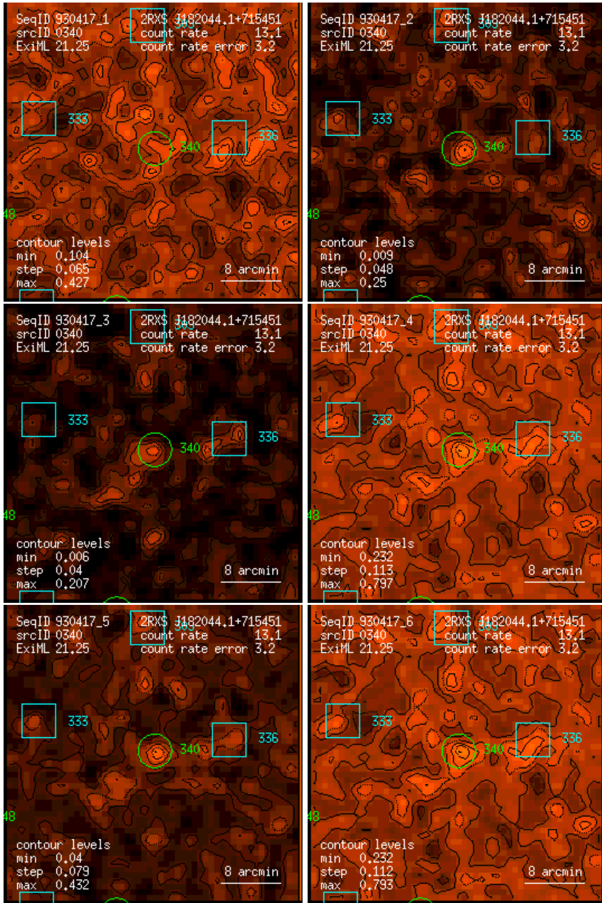
Figure 340: RASS 930417: detection 0340: band rate images, Gaussian filter: (1) PSPC channels 11 – 41, (2) 52 – 90, (3) 91 – 201, (4) 11 – 235, (5) 52 – 201, (6) 11 – 201. Broad band rates in counts/ks. Band rate contour levels in counts/ks/arcmin 2 .
