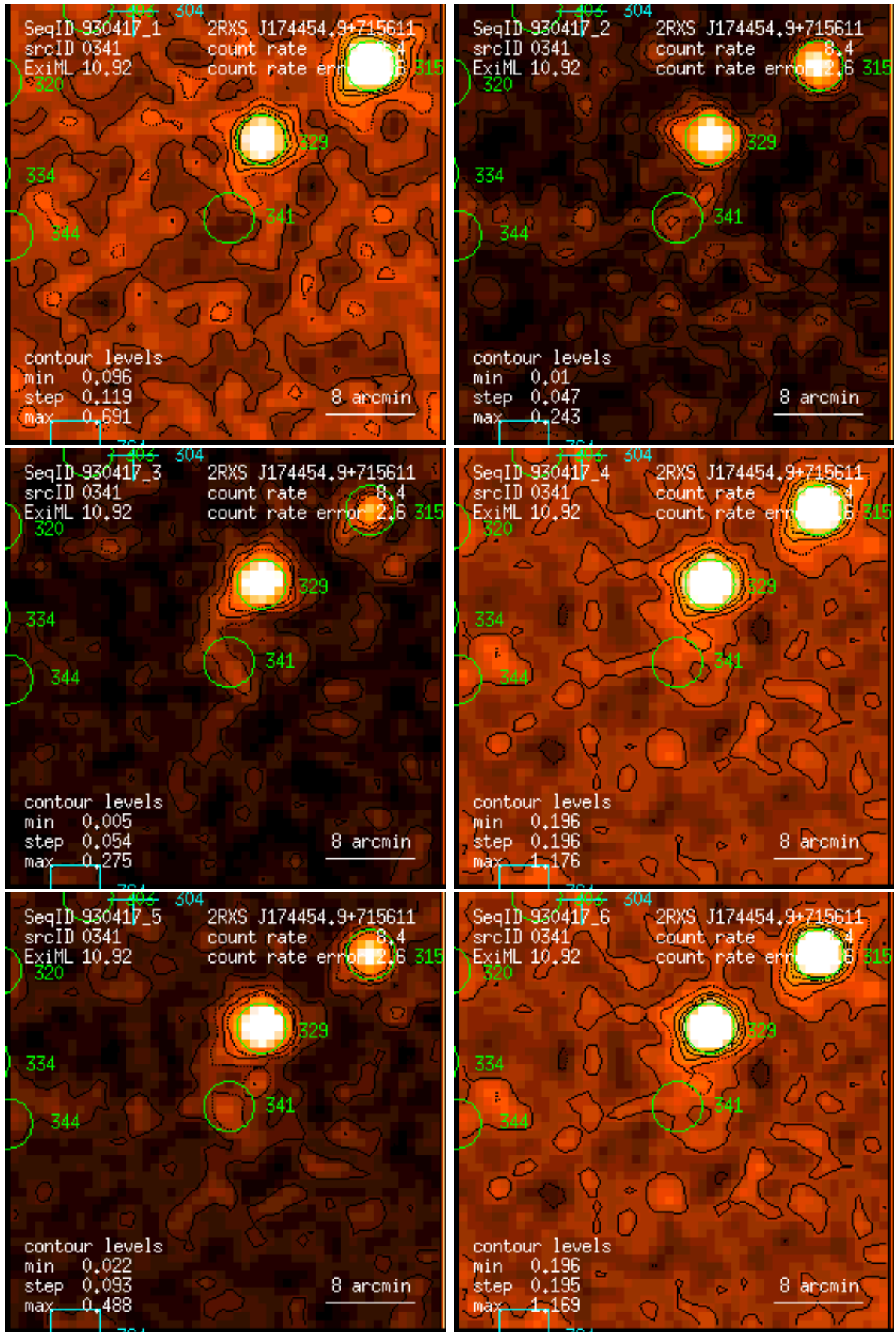
Figure 341: RASS 930417: detection 0341: band rate images, Gaussian filter: (1) PSPC channels 11 – 41, (2) 52 – 90, (3) 91 – 201, (4) 11 – 235, (5) 52 – 201, (6) 11 – 201. Broad band rates in counts/ks. Band rate contour levels in counts/ks/arcmin 2 .
