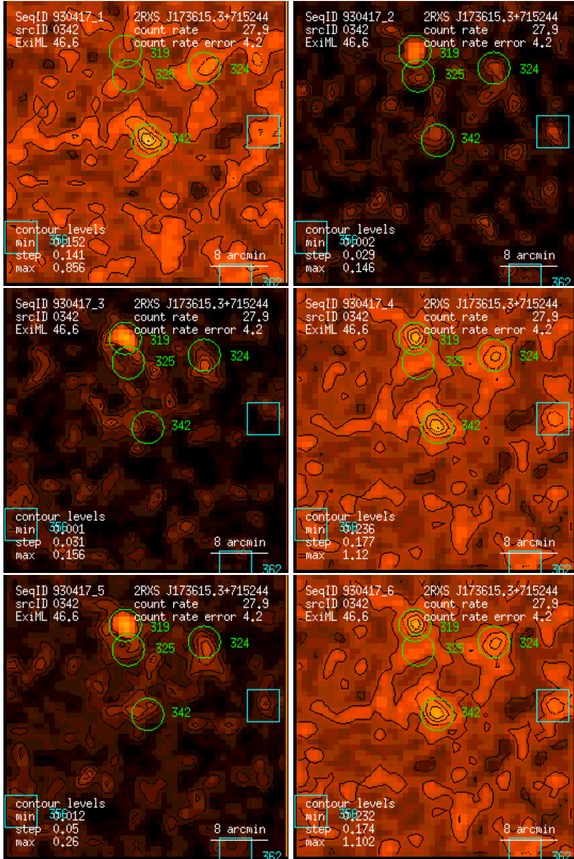
Figure 342: RASS 930417: detection 0342: band rate images, Gaussian filter: (1) PSPC channels 11 – 41, (2) 52 – 90, (3) 91 – 201, (4) 11 – 235, (5) 52 – 201, (6) 11 – 201. Broad band rates in counts/ks. Band rate contour levels in counts/ks/arcmin 2 .
