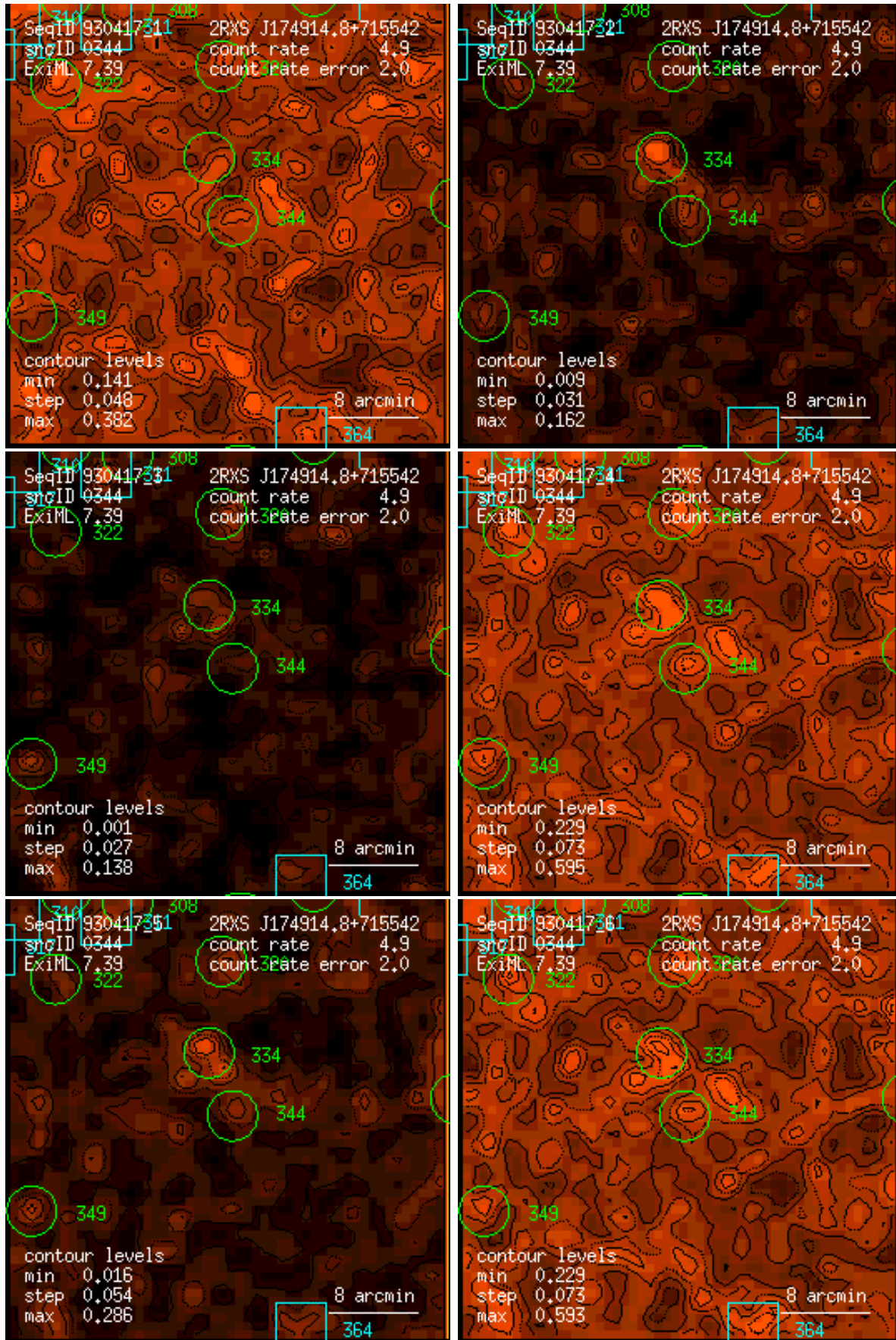
Figure 344: RASS 930417: detection 0344: band rate images, Gaussian filter: (1) PSPC channels 11 – 41, (2) 52 – 90, (3) 91 – 201, (4) 11 – 235, (5) 52 – 201, (6) 11 – 201. Broad band rates in counts/ks. Band rate contour levels in counts/ks/arcmin 2 .
