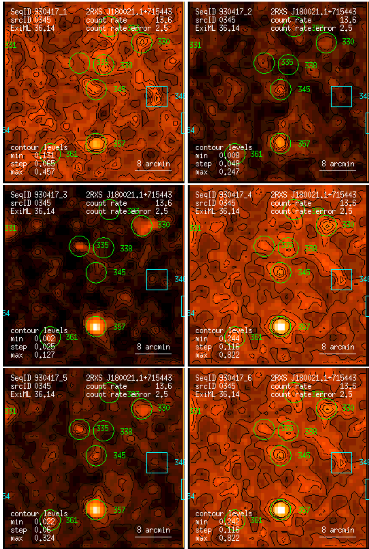
Figure 345: RASS 930417: detection 0345: band rate images, Gaussian filter: (1) PSPC channels 11 – 41, (2) 52 – 90, (3) 91 – 201, (4) 11 – 235, (5) 52 – 201, (6) 11 – 201. Broad band rates in counts/ks. Band rate contour levels in counts/ks/arcmin 2 .
