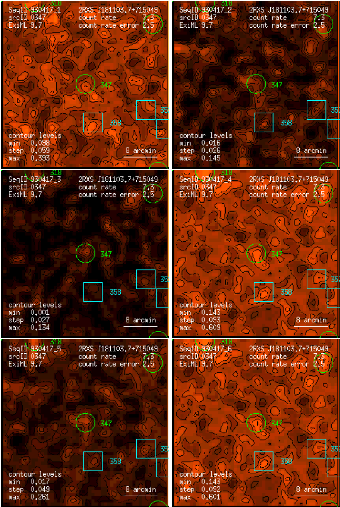
Figure 347: RASS 930417: detection 0347: band rate images, Gaussian filter: (1) PSPC channels 11 – 41, (2) 52 – 90, (3) 91 – 201, (4) 11 – 235, (5) 52 – 201, (6) 11 – 201. Broad band rates in counts/ks. Band rate contour levels in counts/ks/arcmin 2 .
