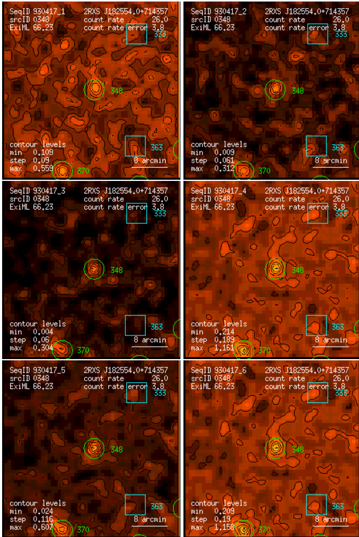
Figure 348: RASS 930417: detection 0348: band rate images, Gaussian filter: (1) PSPC channels 11 – 41, (2) 52 – 90, (3) 91 – 201, (4) 11 – 235, (5) 52 – 201, (6) 11 – 201. Broad band rates in counts/ks. Band rate contour levels in counts/ks/arcmin 2 .
