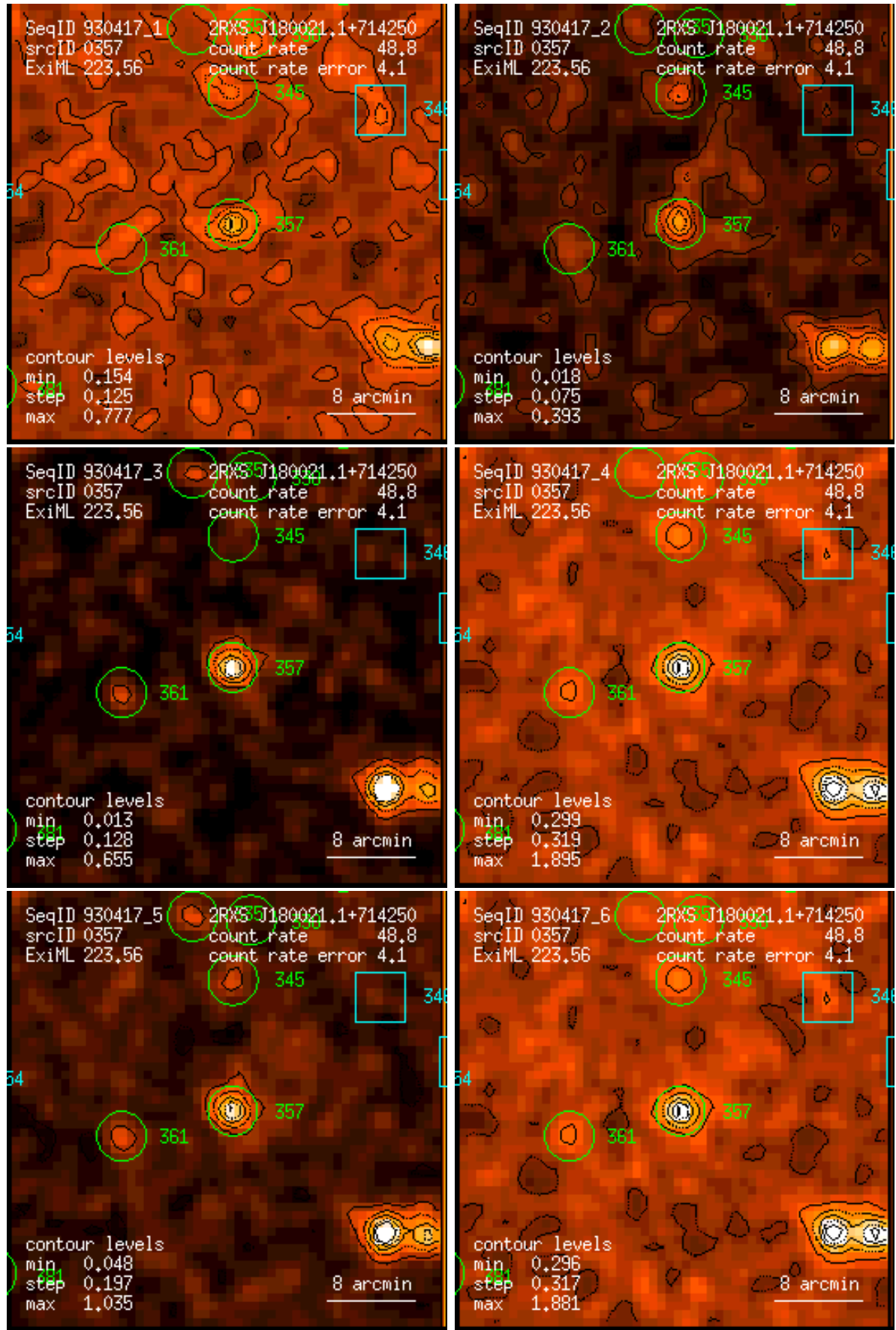
Figure 357: RASS 930417: detection 0357: band rate images, Gaussian filter: (1) PSPC channels 11 – 41, (2) 52 – 90, (3) 91 – 201, (4) 11 – 235, (5) 52 – 201, (6) 11 – 201. Broad band rates in counts/ks. Band rate contour levels in counts/ks/arcmin 2 .
