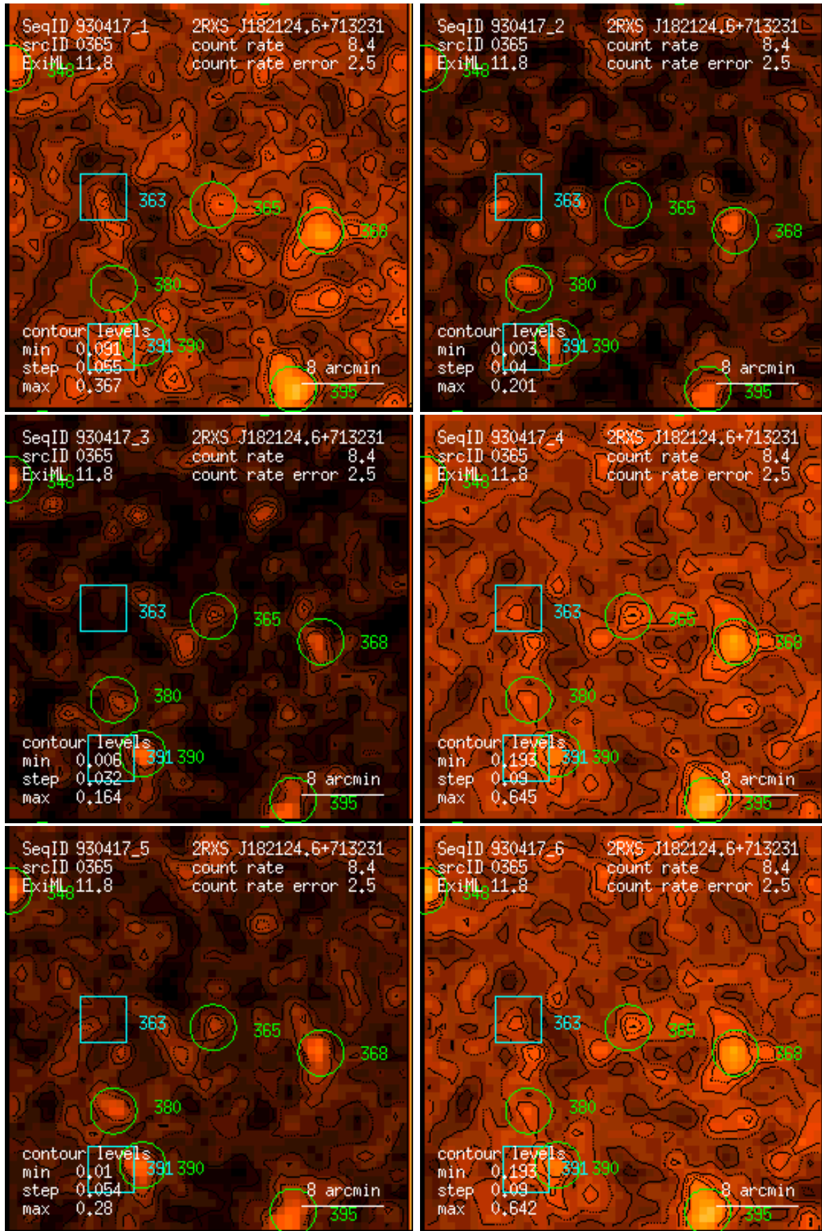
Figure 365: RASS 930417: detection 0365: band rate images, Gaussian filter: (1) PSPC channels 11 – 41, (2) 52 – 90, (3) 91 – 201, (4) 11 – 235, (5) 52 – 201, (6) 11 – 201. Broad band rates in counts/ks. Band rate contour levels in counts/ks/arcmin 2 .
