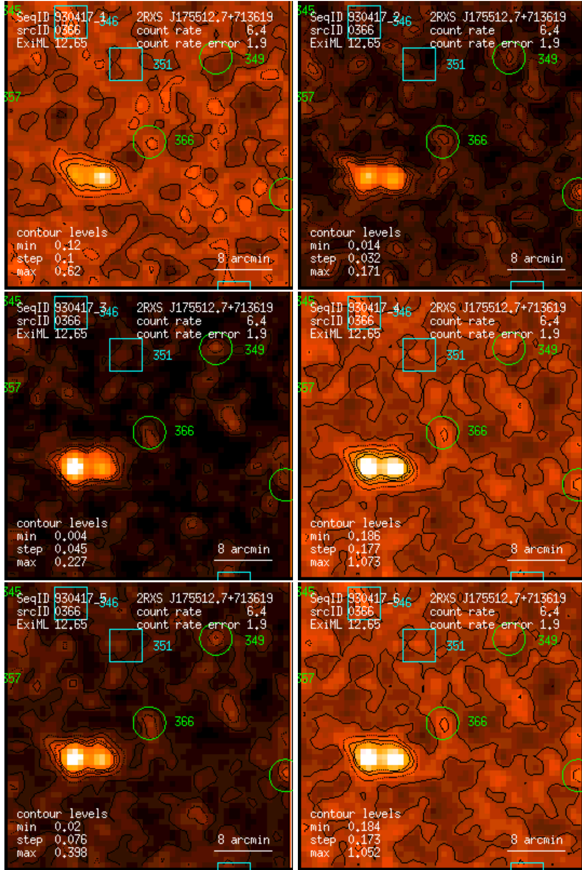
Figure 366: RASS 930417: detection 0366: band rate images, Gaussian filter: (1) PSPC channels 11 – 41, (2) 52 – 90, (3) 91 – 201, (4) 11 – 235, (5) 52 – 201, (6) 11 – 201. Broad band rates in counts/ks. Band rate contour levels in counts/ks/arcmin 2 .
