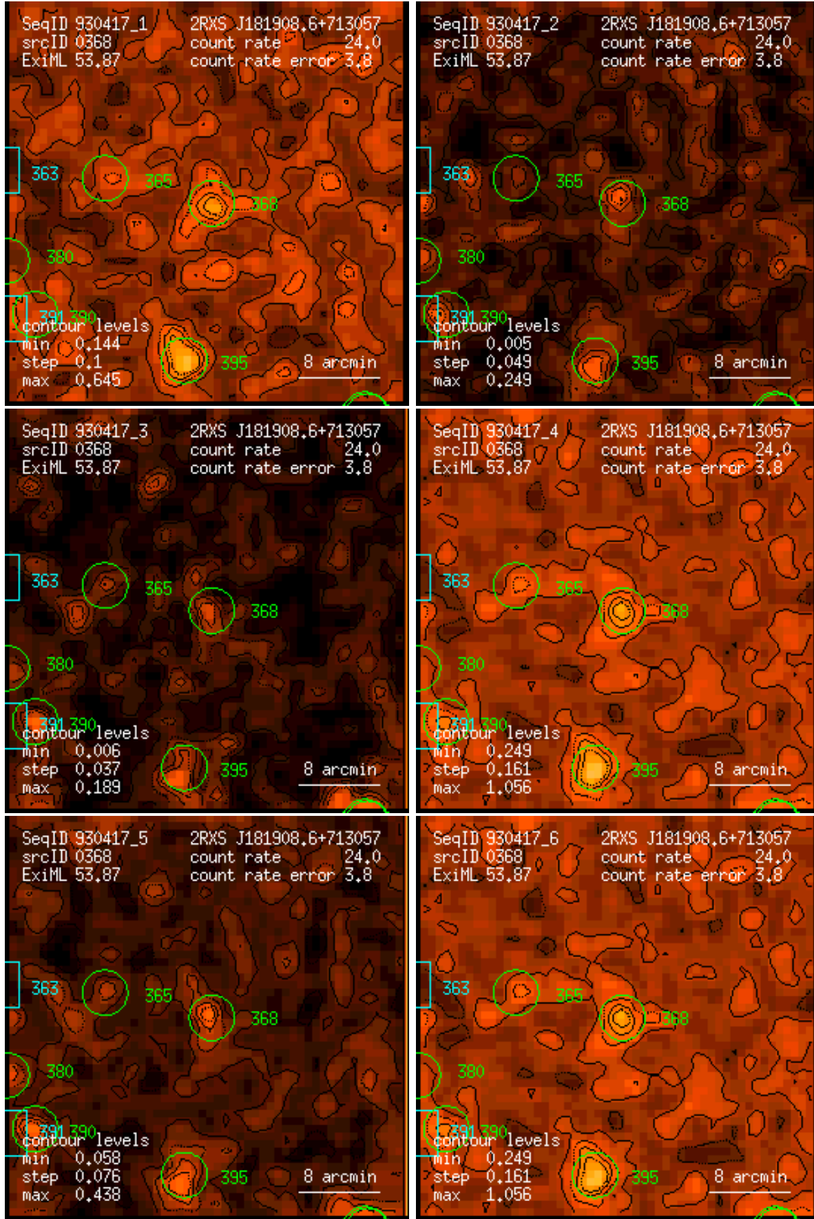
Figure 368: RASS 930417: detection 0368: band rate images, Gaussian filter: (1) PSPC channels 11 – 41, (2) 52 – 90, (3) 91 – 201, (4) 11 – 235, (5) 52 – 201, (6) 11 – 201. Broad band rates in counts/ks. Band rate contour levels in counts/ks/arcmin 2 .
